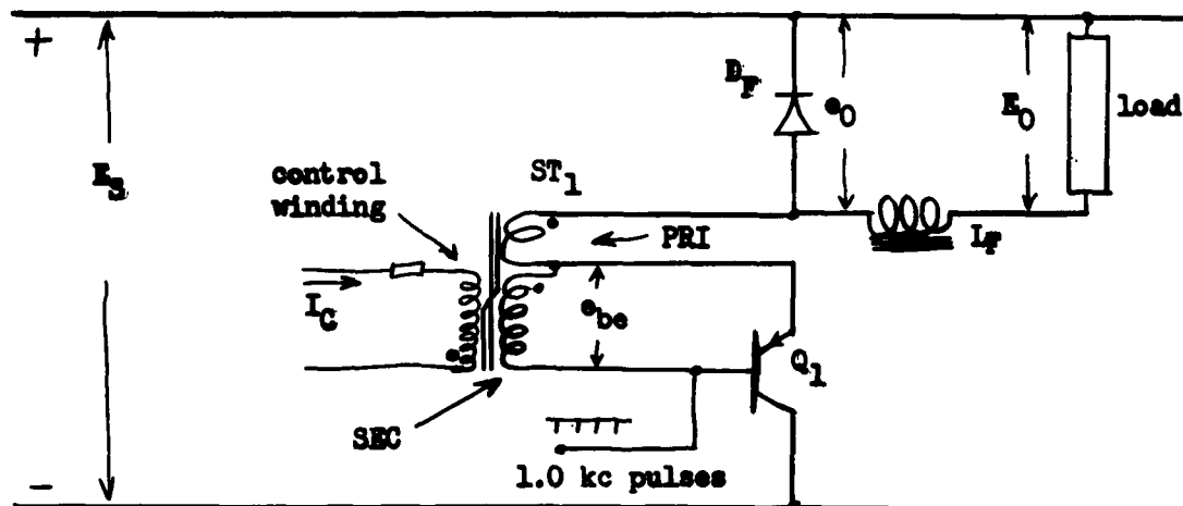
Figure 5.3-18 Control circuit that operates same as Figure 5.3-17 except E_O < E_S in contrast to E_O \geq E_S of Figure 5.3-17. This circuit is unstable if E_O \geq 0.5E_S . The operation of Q_1 and ST_1 is related to I_C same as in Figure 5.3-17. Here E_O/E_S is a direct function of the ratio of time Q_1 is "on" and independent of load current if the voltage drops of Q_1 and D_F are neglected. It is easier to understand the instability in this circuit but the solution applies equally to Figure 5.3-17.
