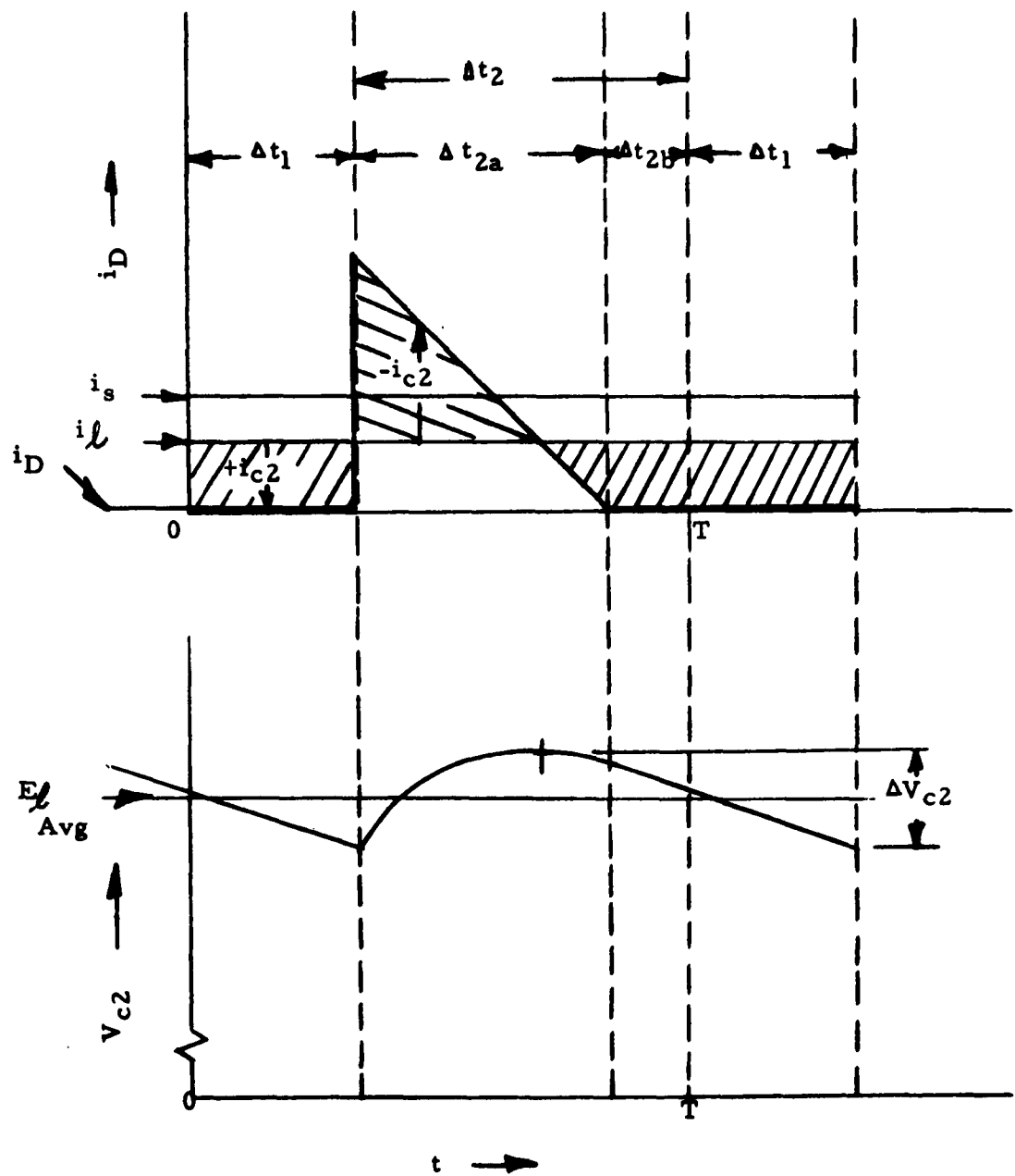
Figure 5.3-9 Light Load Wave Forms -68-
