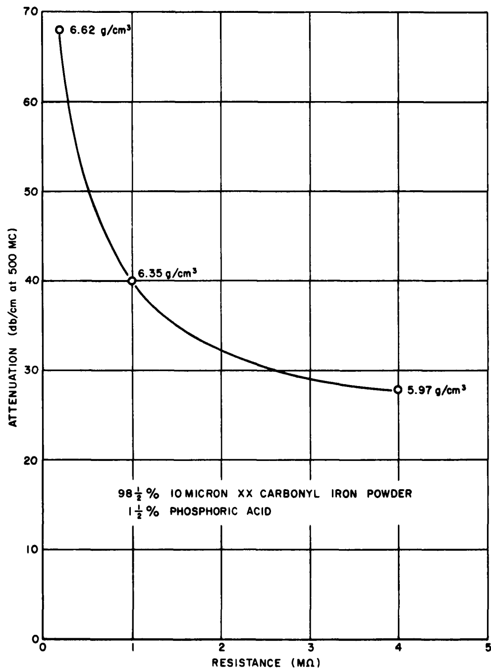
FIG. 3-9. RESISTANCE VERSUS ATTENUATION
