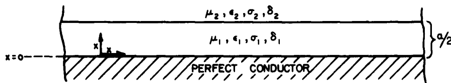
FIG. 2-19. A CONFIGURATION EQUIVALENT TO FIG. 2-18. FOR TM WAVES
