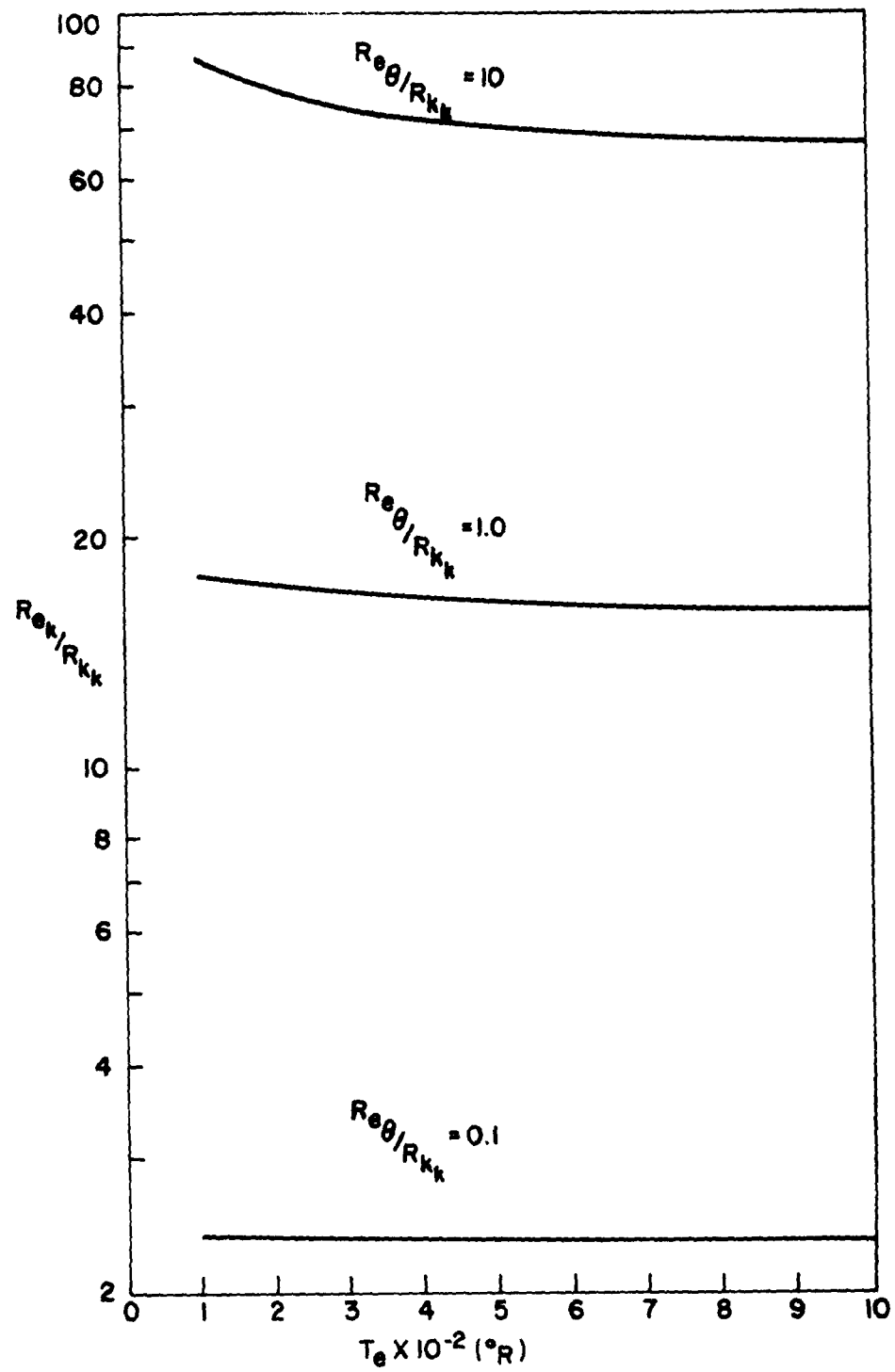
FIG. 2 VARIATION OF ROUGHNESS REYNOLDS NUMBER WITH LOCAL TEMPERATURE
