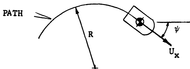
FIGURE 4-9. COORDINATED TURN
