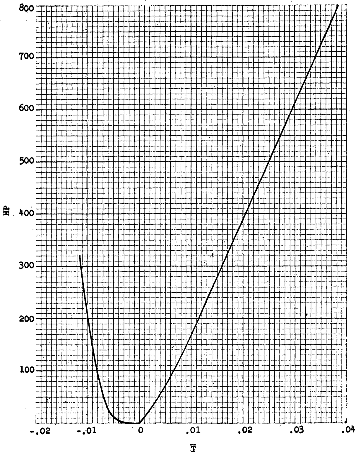
FIGURE 2-4. DRIVING HORSEPOWER VS THRUST
