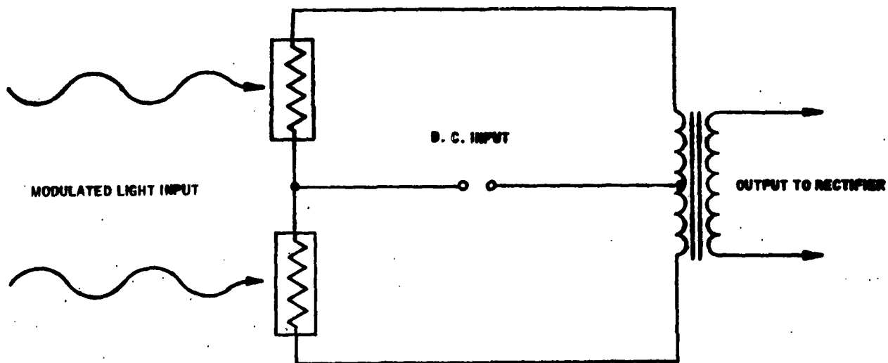
Figure 36 - BASIC PHOTOCONDUCTIVE SWITCHING CIRCUIT
