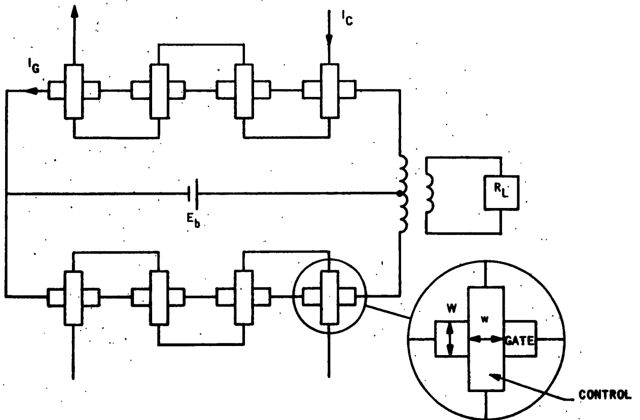
Figure 34 - APPLICATION OF CROSSED-FILM CRYOTRON TO VOLTAGE CONVERSION
