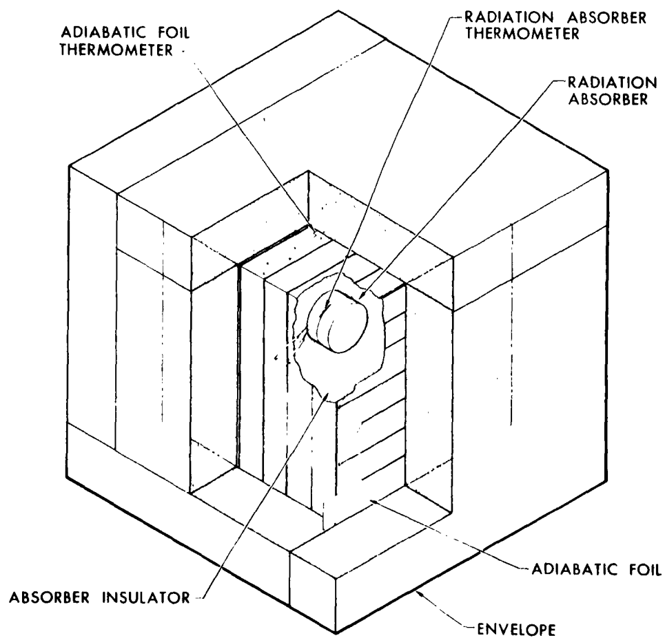
FIGURE 3. ADIABATIC CALORIMETER.
