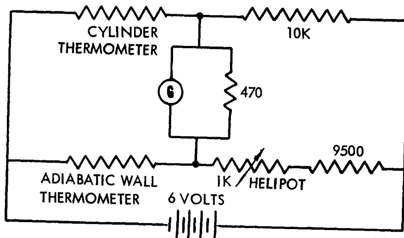
FIGURE 4. (a) BRIDGE FOR TEMPERATURE MEASUREMENT. (b) BRIDGE FOR TEMPERATURE DIFFERENCE DETECTION.
