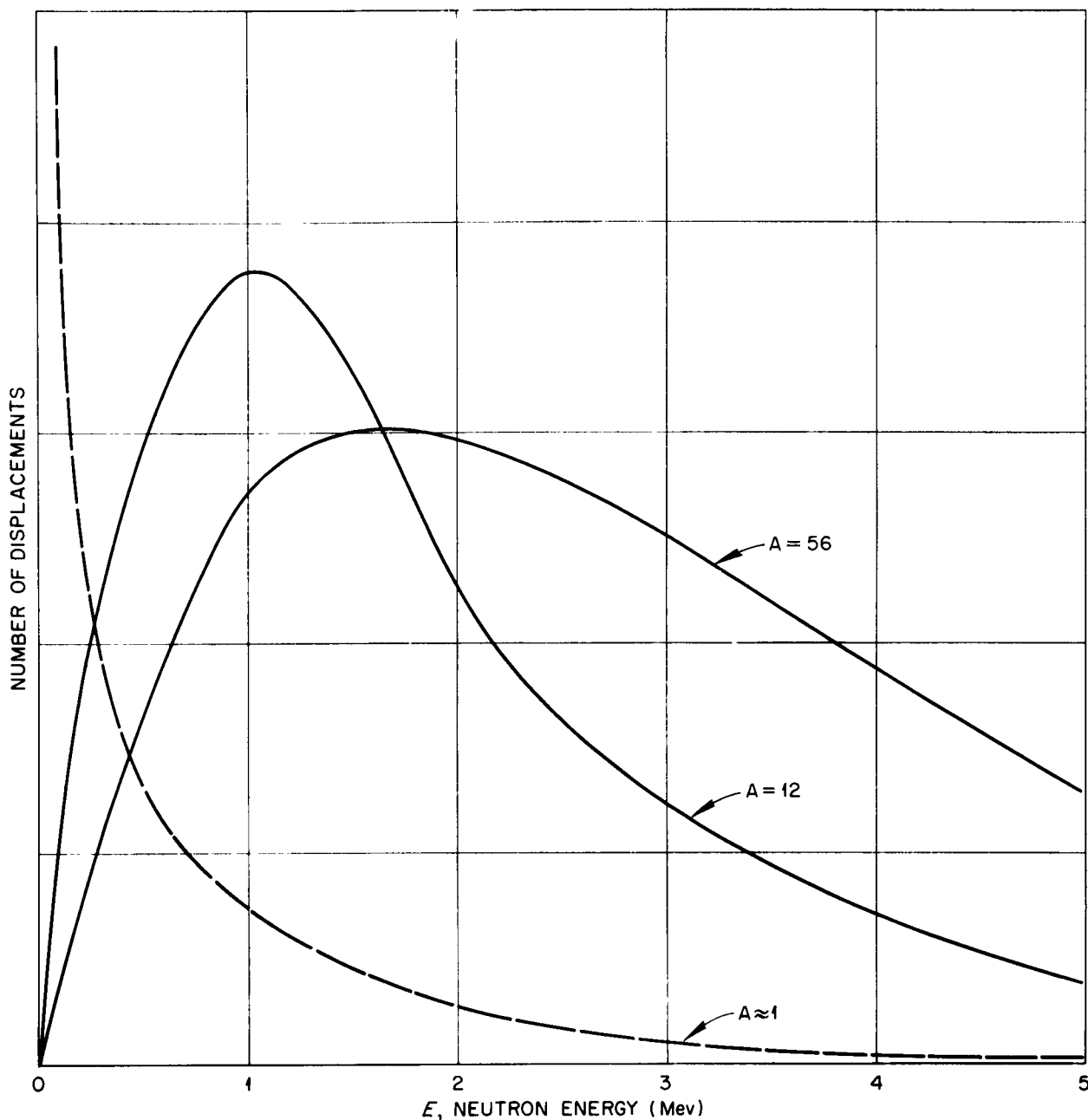
Fig. 6. Displacement production by neutrons. Three curves are shown for the number of displacements, N_d , produced in materials of different A per cc per unit time by neutrons of energy, E . The number of displacements produced by a single neutron, G(E) , was determined from the formulation of Snyder and Neufeld (See text 1). The neutron spectrum was taken from Fig. 3. The curve for A = 1 was calculated assuming G(E) = \text{const} . The scale for the number of displacements is arbitrary and is not the same for all the curves.
