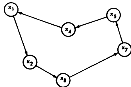
e. A simple cycle
