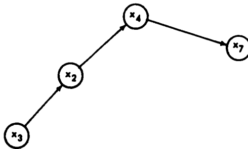
c. A simple x_3 \rightarrow x_7 path
