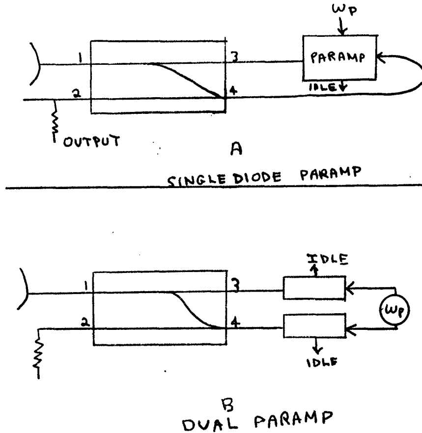
Figure 4-21. Hybrid-Coupled Amplifier
