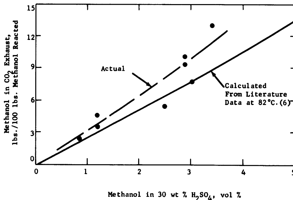
Figure C-4 Methanol Condensed From CO_2 Exhaust Stream
