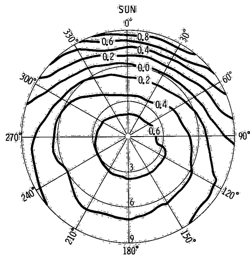
Figure 21. Isoluminance diagram, sky no. 17, 62^{\circ} 05' N , 169^{\circ} 56.1' W , snow covered ice, clear, sun elevation -5.5^{\circ} .
