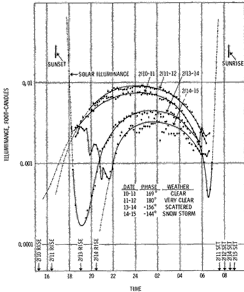
Figure 4. Moon influenced illuminance.
