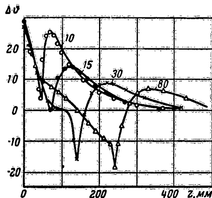
Fig. 62. \Delta T(z) for benzine for various times (run 30).
