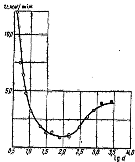
Fig. 24. Relation of v to d for tractor kerosene.
