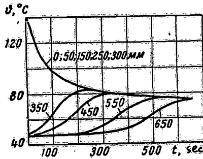
Fig. 36. Temperature as a function of time for various depths in benzine sprayed with water.
