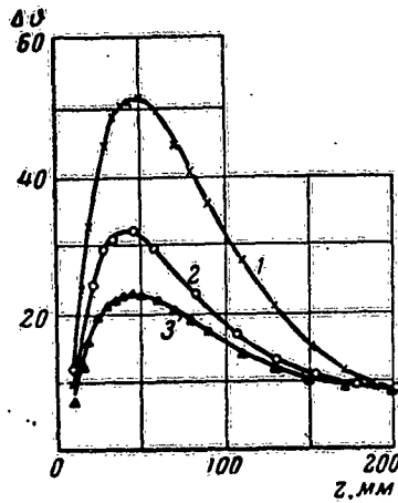
Fig. 50. \Delta v^l(z) for tractor kerosene ( d = 150 mm); w , m/sec: 1) 2.6; 2) 1.8; 3) 1.15.
