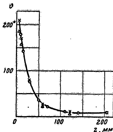
Fig. 43. \vartheta^l = f(z) for tractor kerosene
