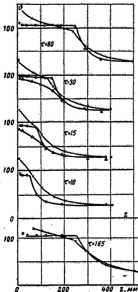
Fig. 55. Temperature distribution in the liquid and at the wall for automobile gasoline at various times: O liquid, x wall. The times \tau are in minutes.
