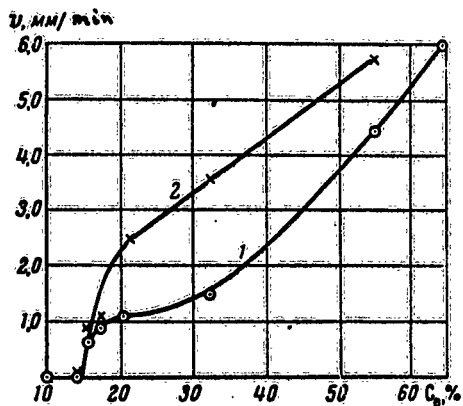
Fig. 30. Relation of v to c_0 : 1) diesel oil; 2) benzene.
