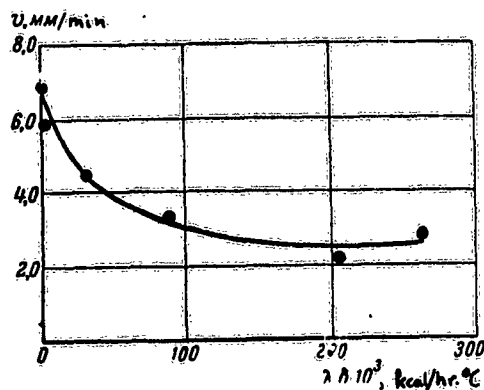
Fig. 22. Relation of v to \lambda h for benzine.
