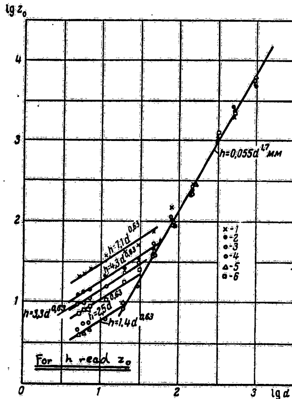
Fig. 37. Relation of z_0 to d for various fuels: 1) automobile benzine; 2) tractor kerosene; 3) illuminating kerosene; 4) transformer oil; 5) solar oil; 6) diesel oil.
