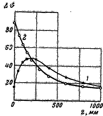
Fig. 51. \Delta v^l(z) for kerosene ( d = 1300 mm); w , m/sec: 1) 1.4; 2) 1.0.
