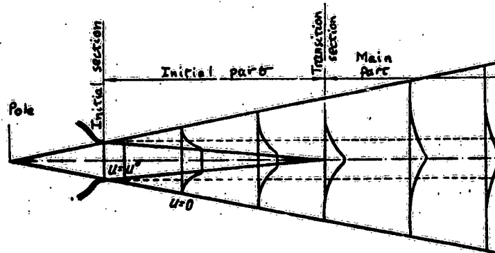
Fig. 2. Jet entering a body of fluid.
