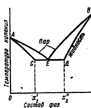
Fig. 23: Boiling point of infinitely soluble liquids v. phase composition for constant pressure. Ord.: b.p.; absc.: composition; center: vapor; diag.: liquid.
