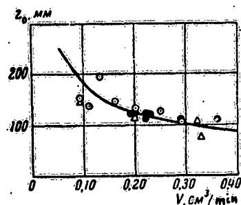
Fig. 2. Relation of z_0 to rate of consumption of liquid.
