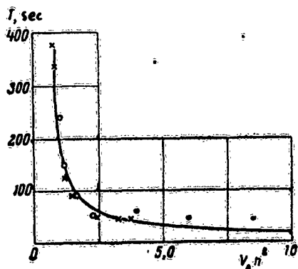
Fig. 20. Relation of T to h^2 V_0 .
