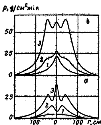
Fig. 29. Relation of flow density to distance from axis of spray for jets of d , equal to 1, 2, and 3 mm: a) p = 5 atm; b) p = 10 atm.
