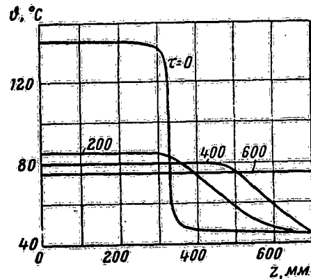
Fig. 37. Temperature as a function of depth for various times during the spraying of benzine with water.
