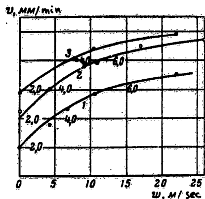
Fig. 32. Relation of v to wind speed: 1) tractor kerosene, d = 300 mm; 2) the same, d = 490 mm; 3) diesel oil, d = 490 mm.
