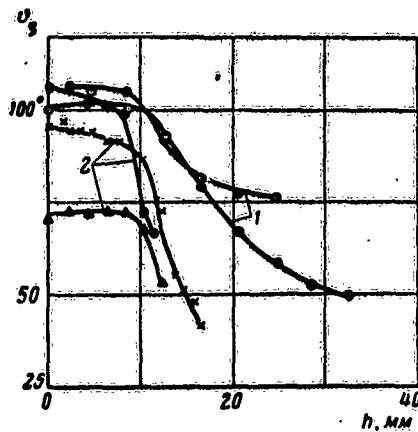
Fig. 34. Relation of \phi_s to change in level: \odot and x , benzine; \Delta , ethanol; + and \bullet , butanol; 1) d = 23 mm; 2) d = 11 mm.
