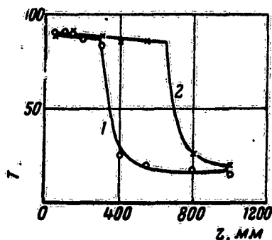
Fig. 54. Temperature distribution in burning benzine ( d = 130 cm) after 1) 20 min; 2) 40 min.
