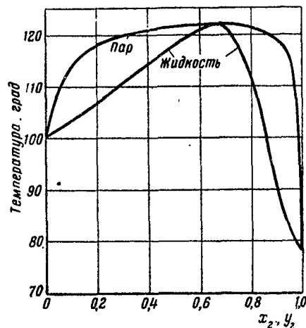
Fig. 20: Dependence of boiling point of mixtures of nitric acid and water on phase composition at constant pressure. Ordinate: temperature, degrees; left: vapor; right: liquid.
