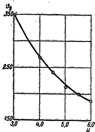
Fig. 40. Surface temperature in relation to the rate of increase in the depth of the homothermal layer for crude petroleum.
