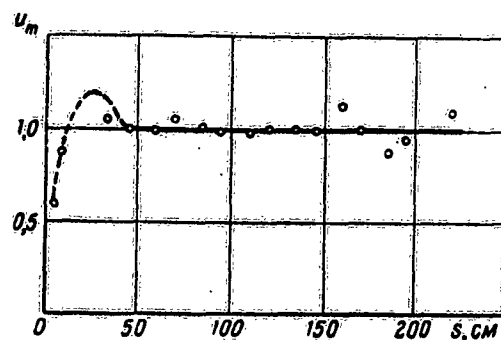
Fig. 15. Velocity at the axis as a function of distance from nozzle.
