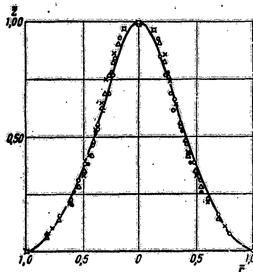
Fig. 4. Shapes of diffusion flames of ethanol in burners.
