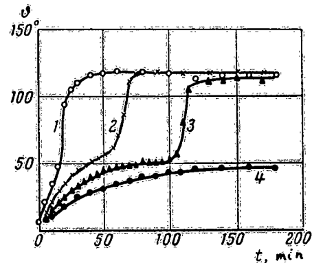
Fig. 42. \tau^\ell = f(t) for benzine; z (mm): 1) 60; 2) 100; 3) 130; 4) 195.
