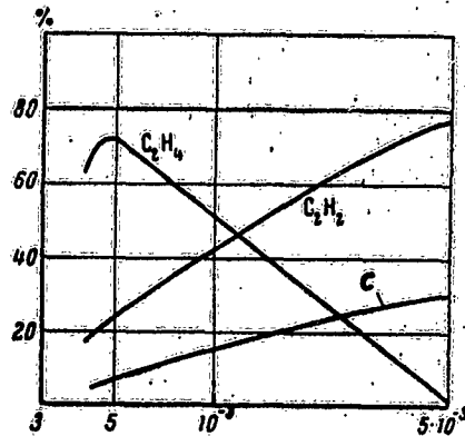
Fig. 11. Pyrolysis products from ethane at 1400^\circ .
