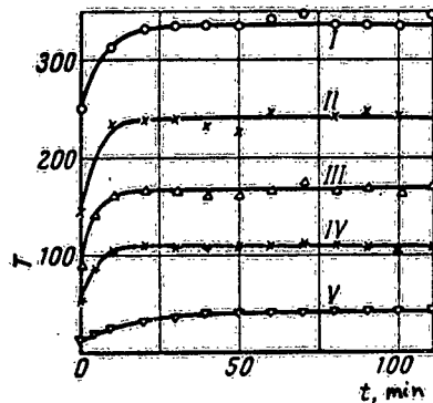
Fig. 41. Relation of \tau^\ell to time for transformer oil; z (mm): I) 0; II) 2; III) 3; IV) 9; V) 29.
