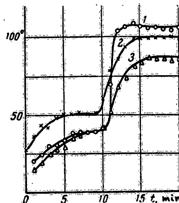
Fig. 63. Temperature vs. time for points in the same plane in benzine: 1) in liquid; 2) lee wall; 3) windward wall.
