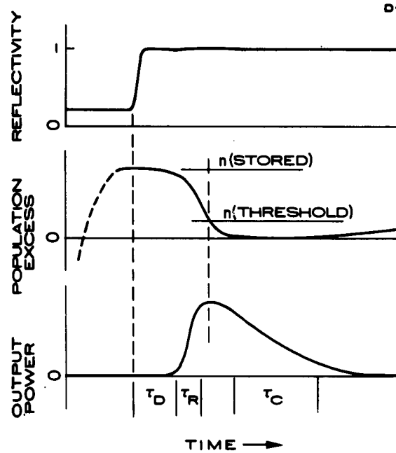
Fig. 1. Typical time sequence of effective reflectivity, population excess n , and output beam power for a giant pulse with fast switching.
