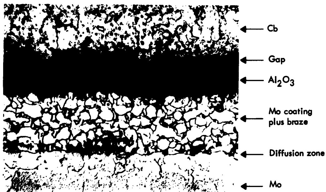
FIGURE 4. Ni-Mo-Fe BRAZE
