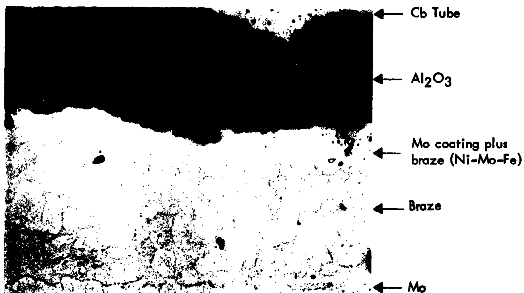
FIGURE 3. Ni-Mo-Fe BRAZE
