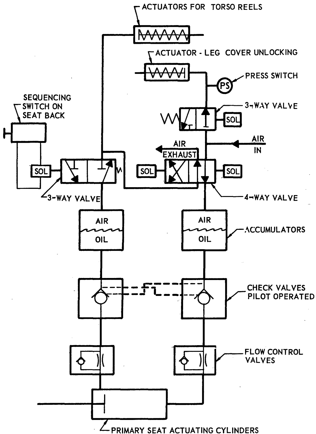
FIGURE 28 POWER SYSTEM SCHEMATIC
