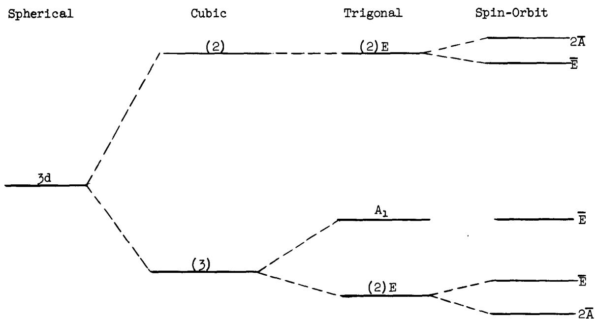
Fig. 11. Split in energy levels upon introduction of perturbations.
