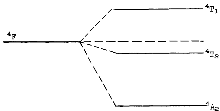
Fig. 13. Splitting of ^4F ground states.
