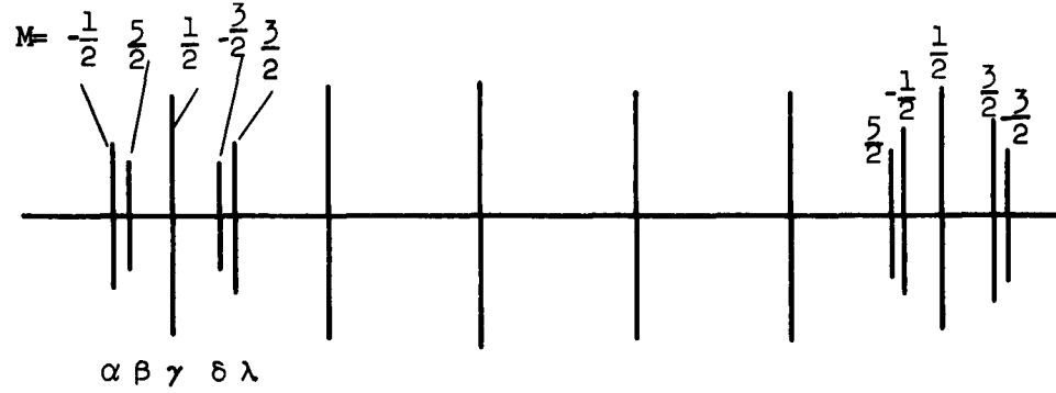
Fig. 18. Schematic plot of fine structure of ESR spectrum of Mn^{++} in cubic ZnS for m = -5/2 and 5/2 .
