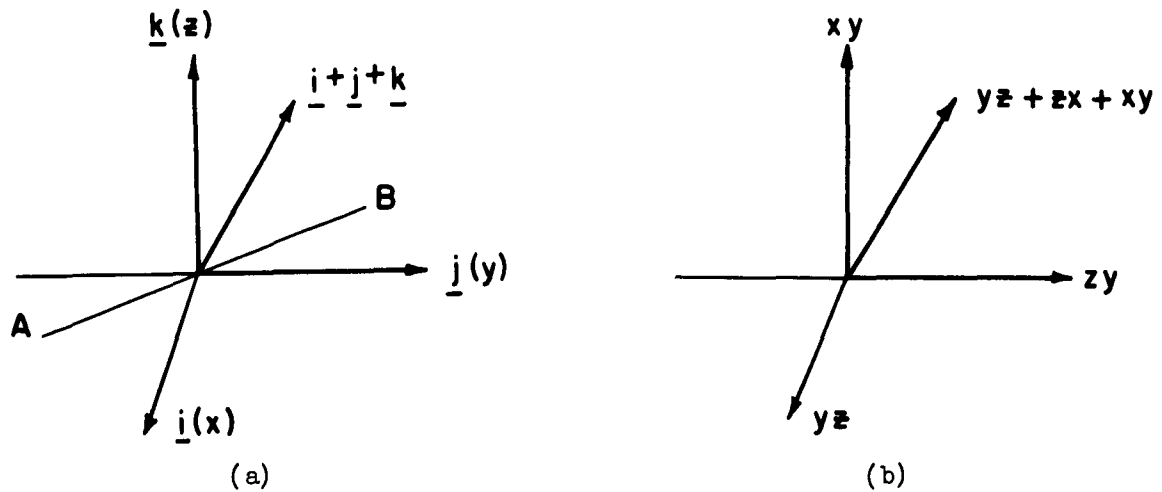
Fig. 9. Geometric constructions of linearly independent functions (simplified).
