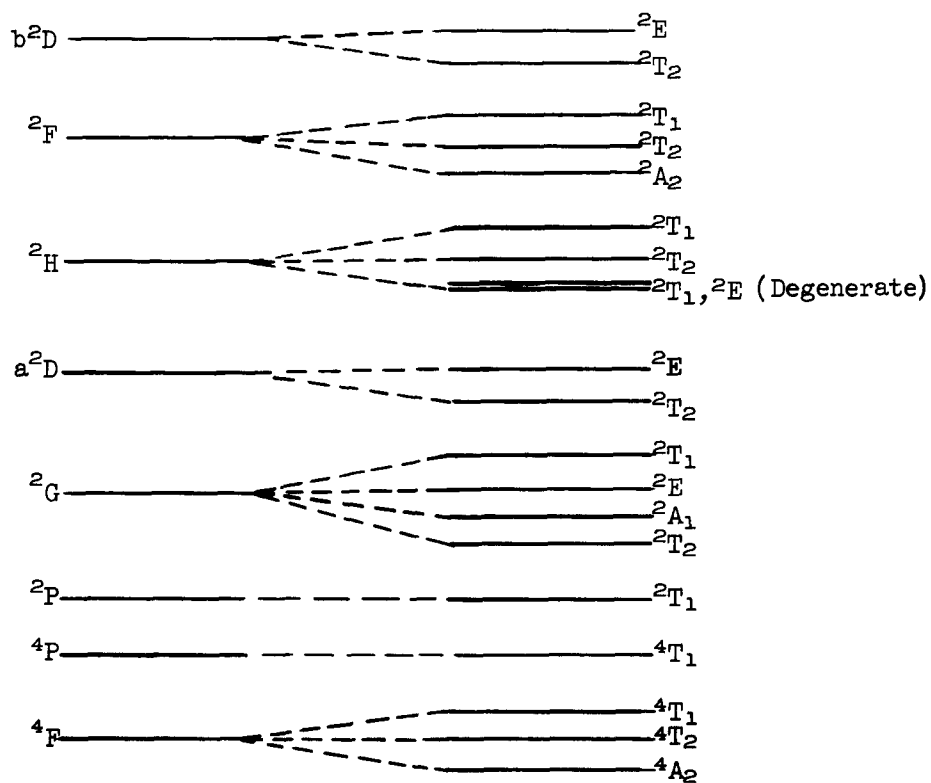
Fig. 14. Complete splitting scheme of the terms arising from the 3d^3 configuration.
