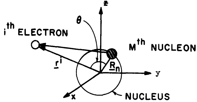
Fig. 10. Schematic representation of electron-nucleon coulomb interaction.
