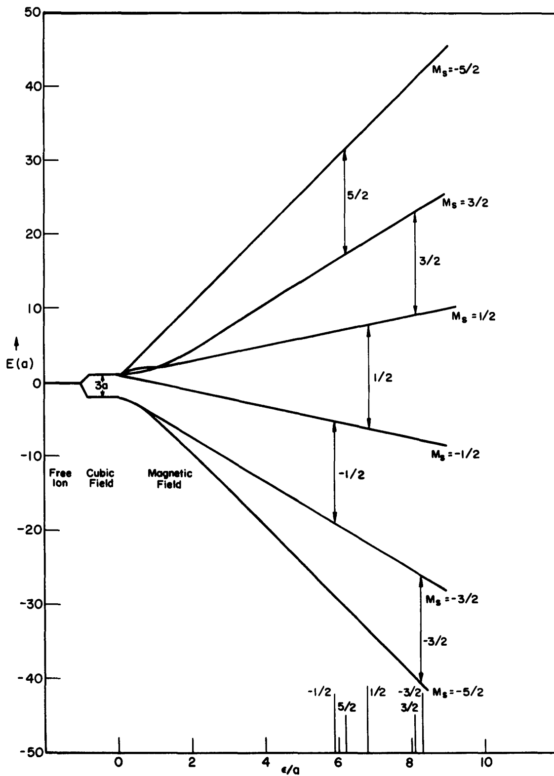
Fig. 15. Energy level scheme of 3d^5 e_g s_{5/2} ( Mn^{++} ) in a tetrahedral field at \theta = 0^\circ .
