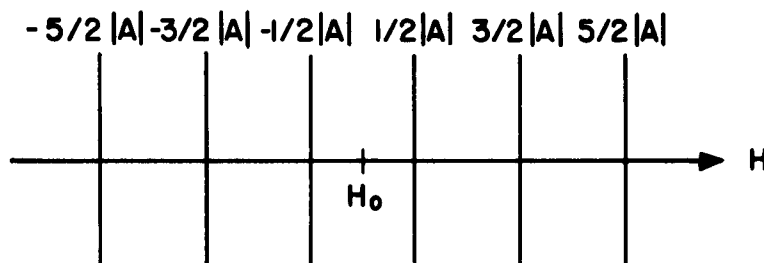
Fig. 13. Theoretical prediction of Mn^{++} ESR spectrum.
