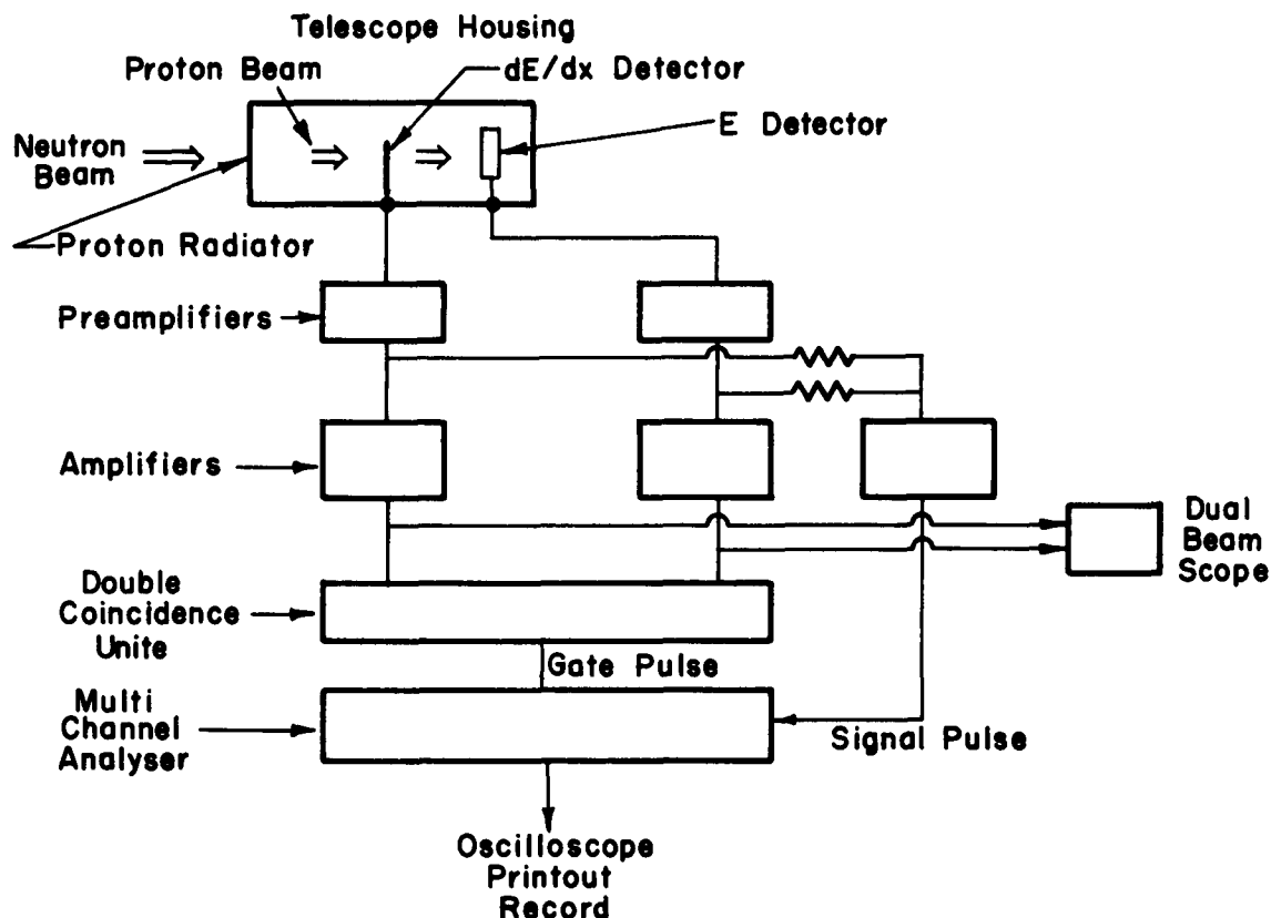
Fig. 1. Block diagram of telescope spectrometer and necessary circuitry for coincidence counting.
