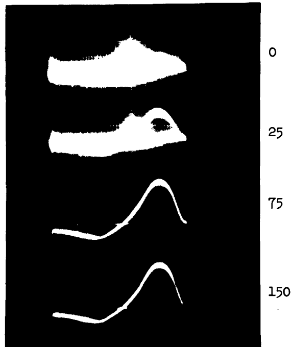
Fig. 4. Pulse shape of large area dE/dx detector to Po^{210} alphas vs. bias across the detector and 22-meg load resistor. Voltage is 0, 25, 75, and 150 volts; the leakage current is over 1 microampere.
