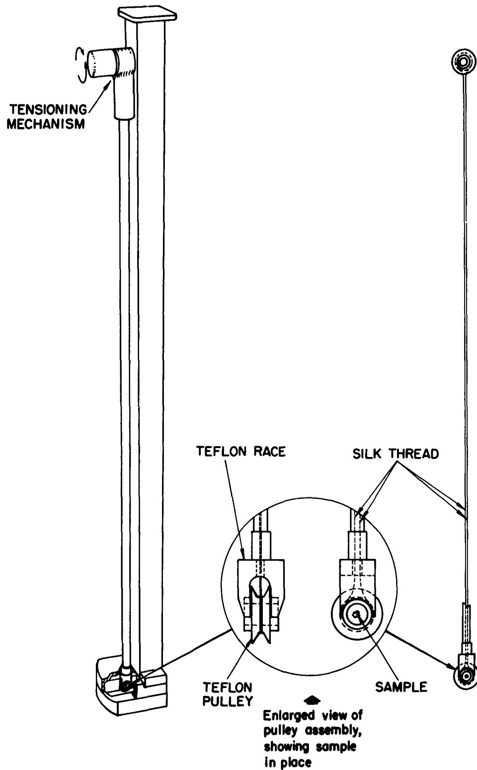
Fig. 2. Rotating sample holder and resonance cavity used for measurements.
