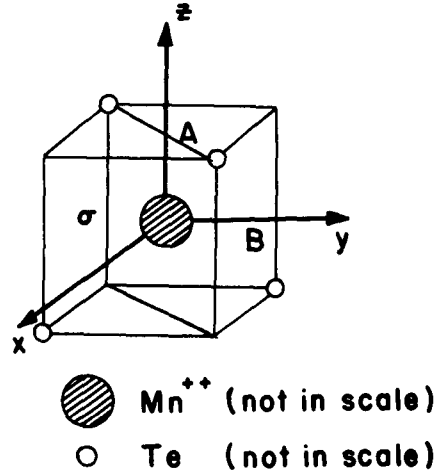
Fig. 12. A unit cell of cubic ZnTe single crystal showing a Mn^{++} ion surrounded by four Te ions and the reflection planes \sigma .
