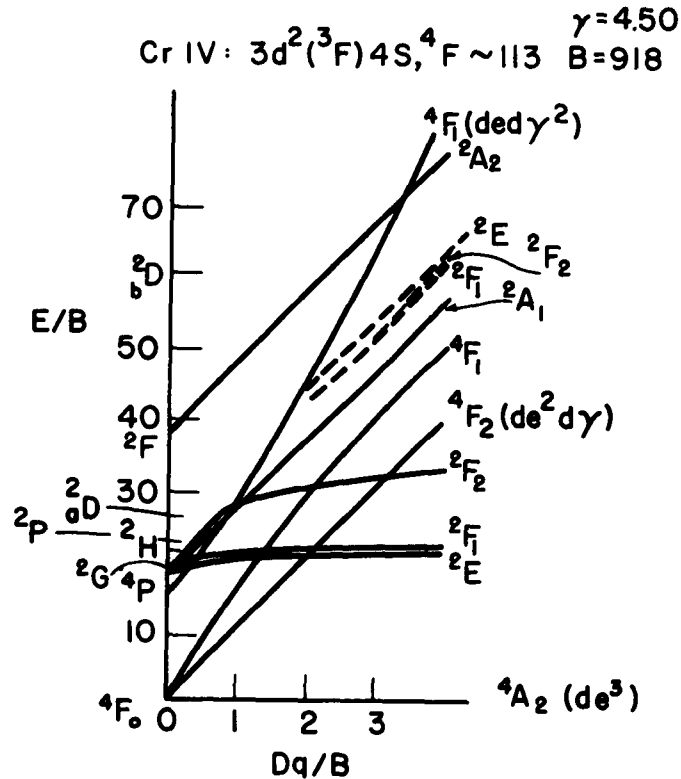
Fig. 12. Splitting of states of the 3d^3 configuration by an octahedral field (Ref. 5, Fig. 2).
