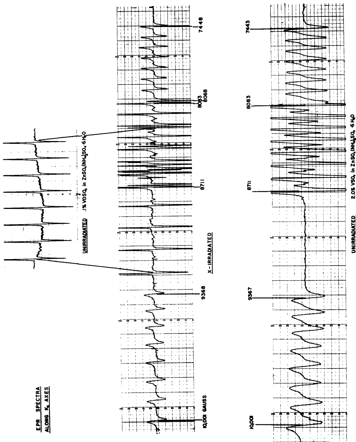
Fig. 1. EPR spectra along K_2 axes.
