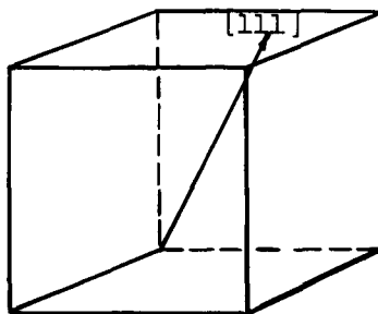
Fig. 8. Cube with [111] body diagonal.
