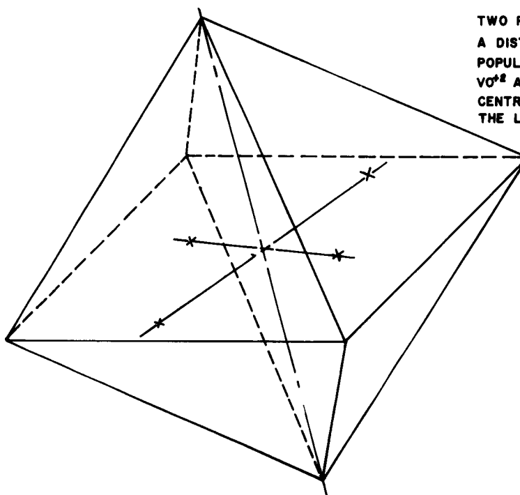
Fig. 7. Experimental positions of axes in \text{VO}(\text{NH}_4)_2(\text{SO}_4)_2 \cdot 6\text{H}_2\text{O} (1% VO/Zn).
