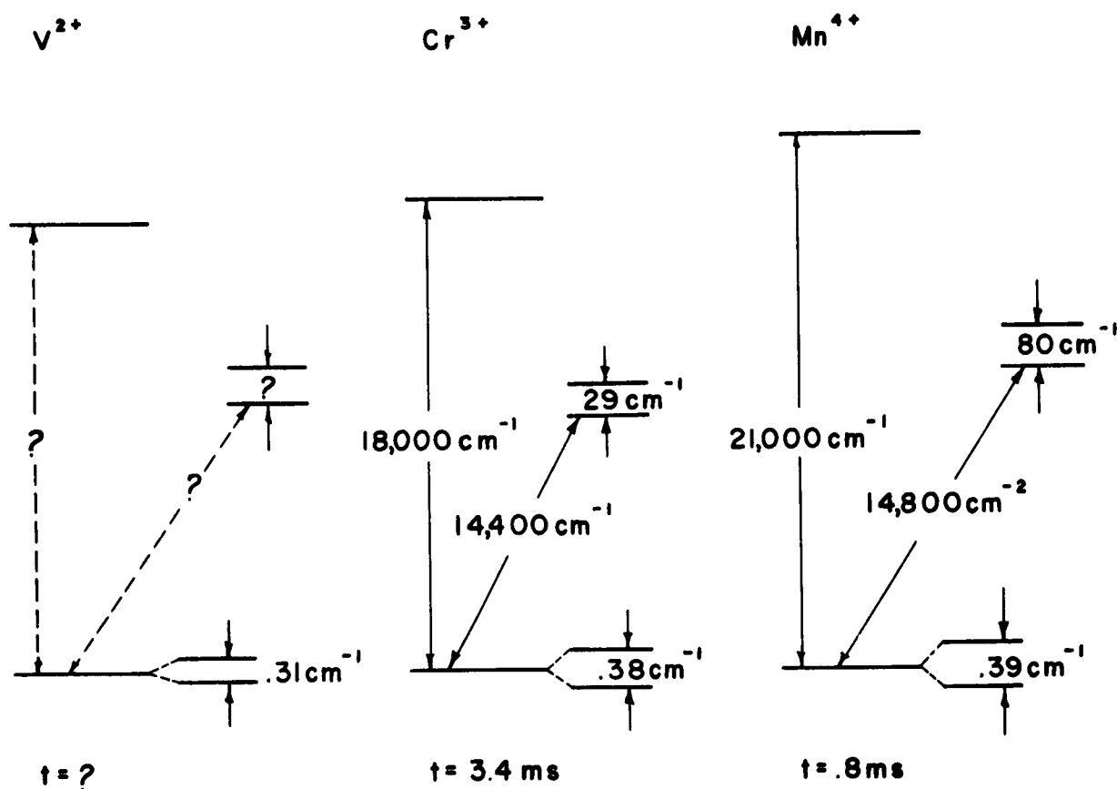
Fig. 6. Properties of \text{V}^{2+} , \text{Cr}^{3+} , and \text{Mn}^{4+} .
