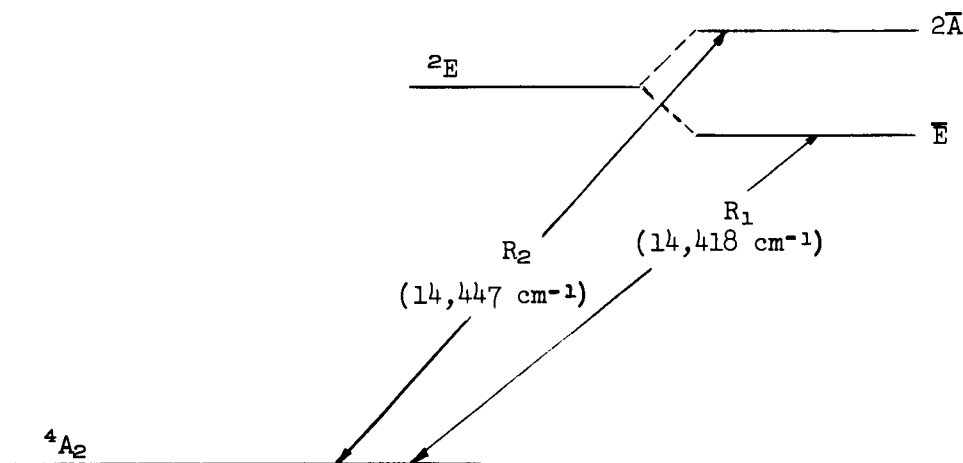
Fig. 4. Split in {}^2E level by trigonal field.
