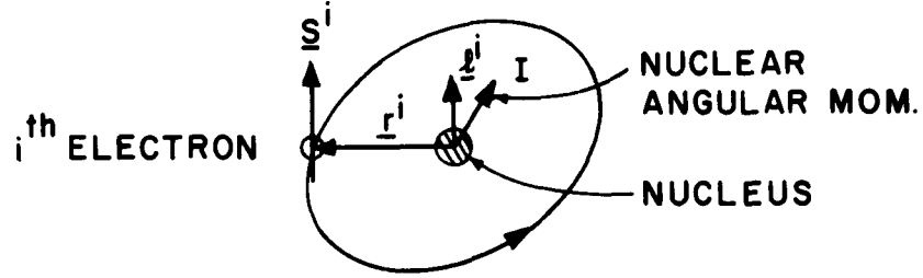
Fig. 9. Schematic representation of electron-nucleus magnetic interaction.
