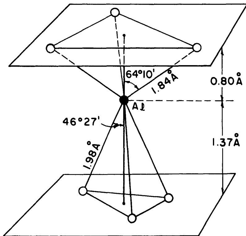
Fig. 1. Coordination of Al atom in \alpha\text{-Al}_2\text{O}_3 .
