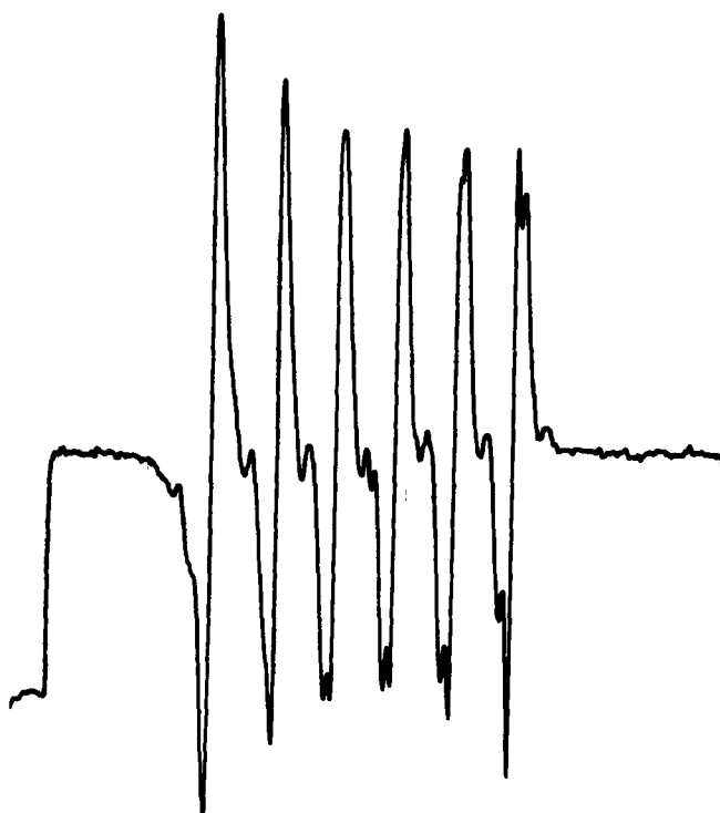
Fig. 7. \text{Mn}^{++} ESR spectrum in CdTe single crystals at 4.2^\circ\text{K} , \theta = 30^\circ .
