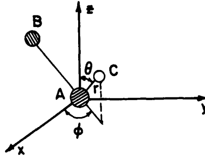
Fig. 11. Schematic representation of crystalline field. (A is the ion, B is its closest neighbor, and C is its electron.)
