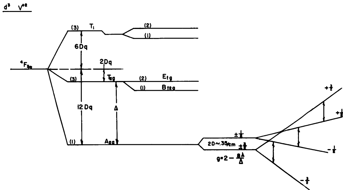
Fig. 2. V^{3+} and V^{2+} energy levels.
