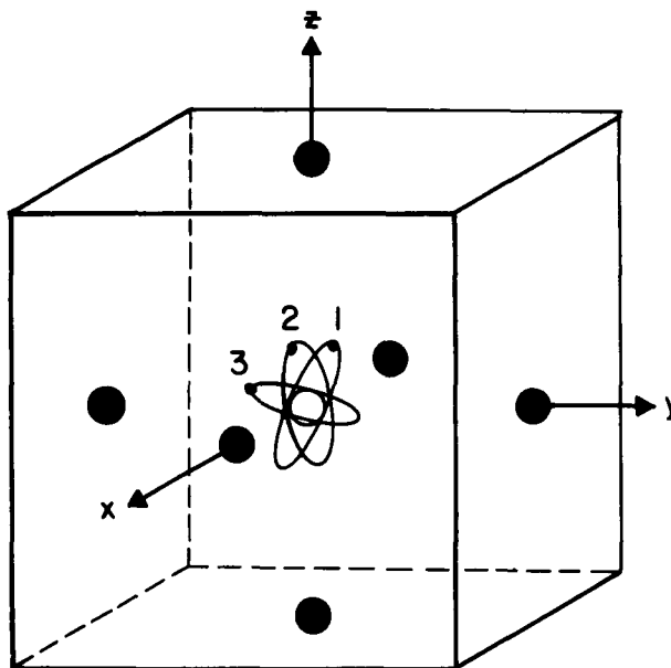
Fig. 7. Octahedral coordination.
