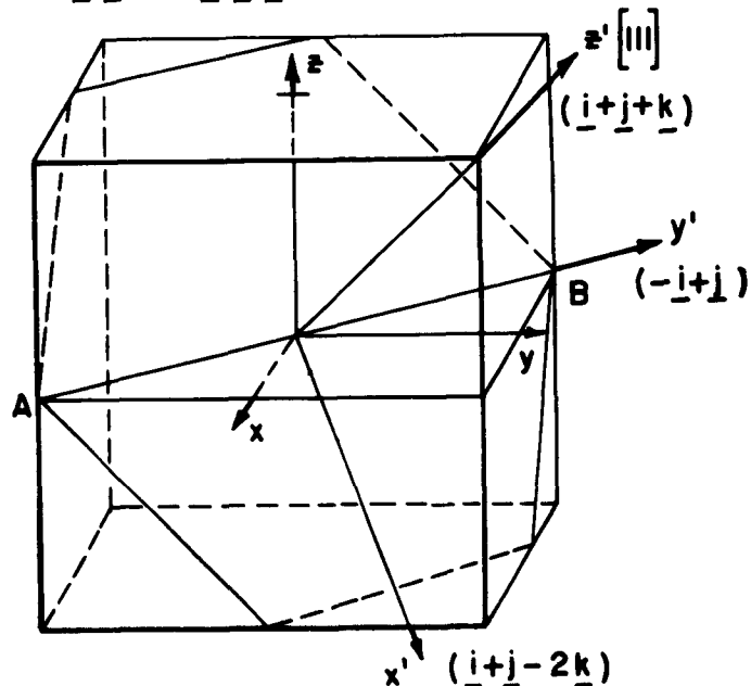
Fig. 10. Geometric constructions of linearly independent functions.
