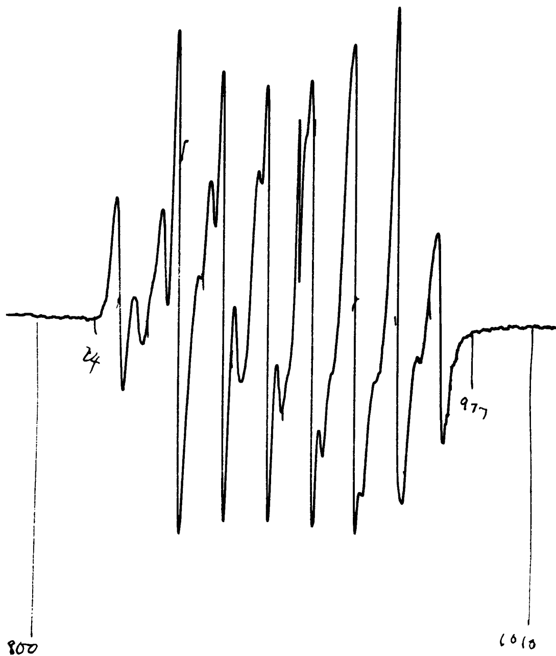
Fig. 6. \text{Mn}^{++} ESR spectrum in CdTe single crystals at 78^\circ\text{K} , \theta = 0^\circ .
