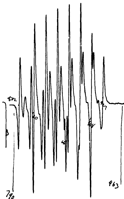
Fig. 8. \text{Mn}^{++} ESR spectrum in CdTe single crystals at 4.2^\circ\text{K} , \theta = 0^\circ .
