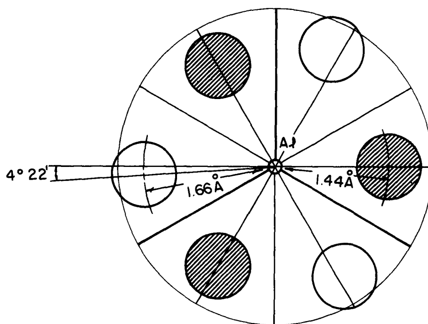
Fig. 2. Projection of oxygens on horizontal plane.
