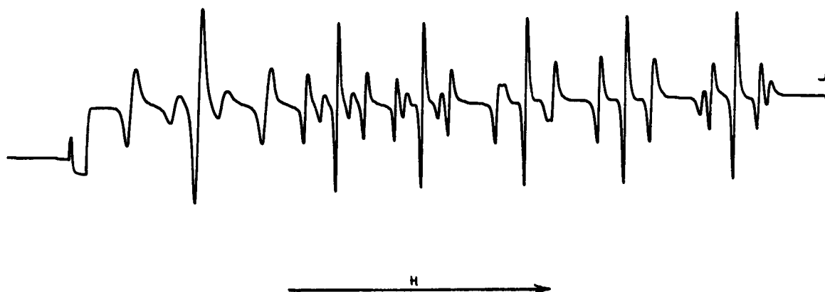
Fig. 16. Mn^{++} ESR spectrum in ZnS (cubic) at 300°K, \theta = 0^\circ .
