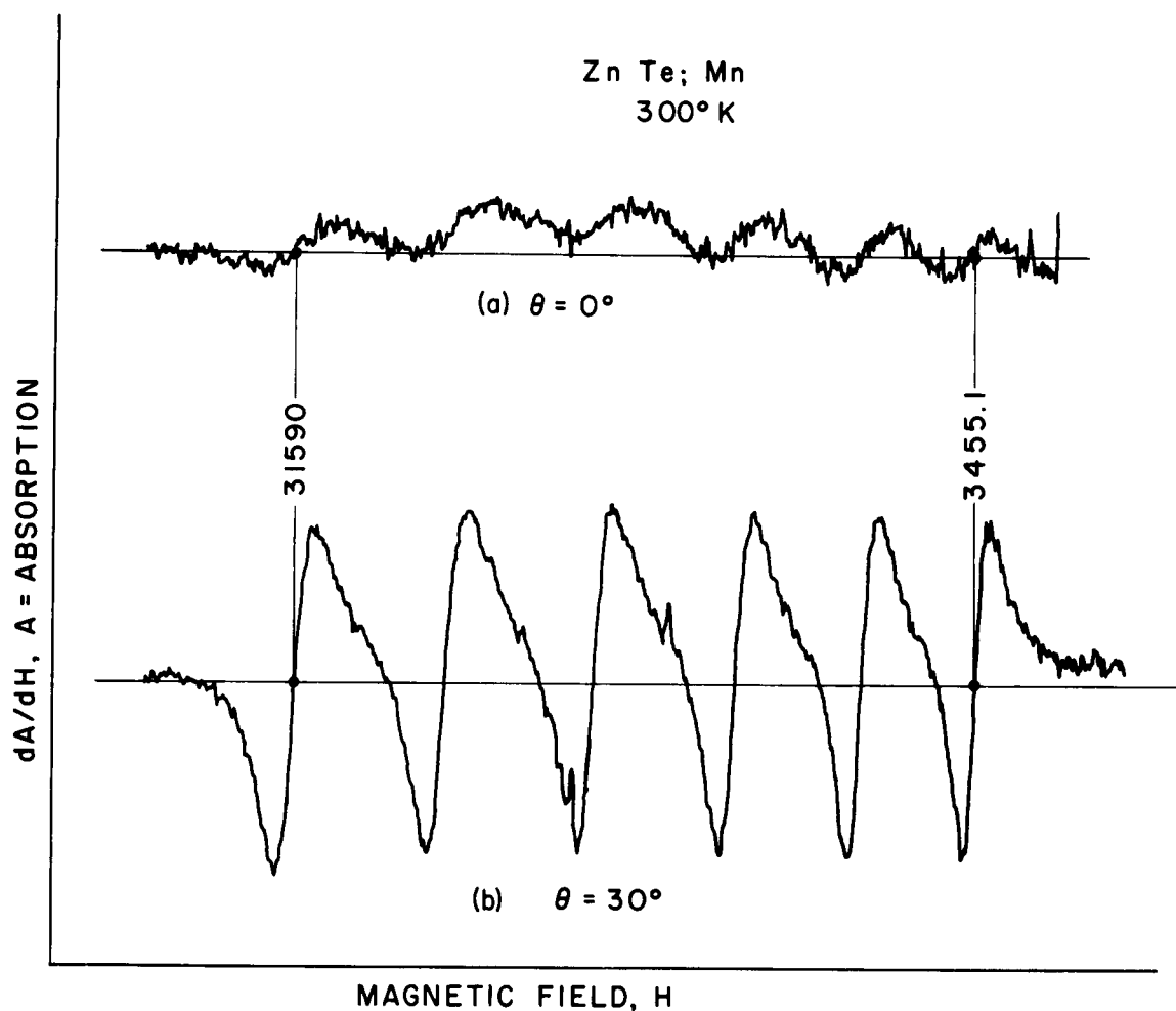
Fig. 3. \text{Mn}^{++} ESR spectrum at 300°K: (a) \theta = 0^\circ ; (b) \theta = 30^\circ .
