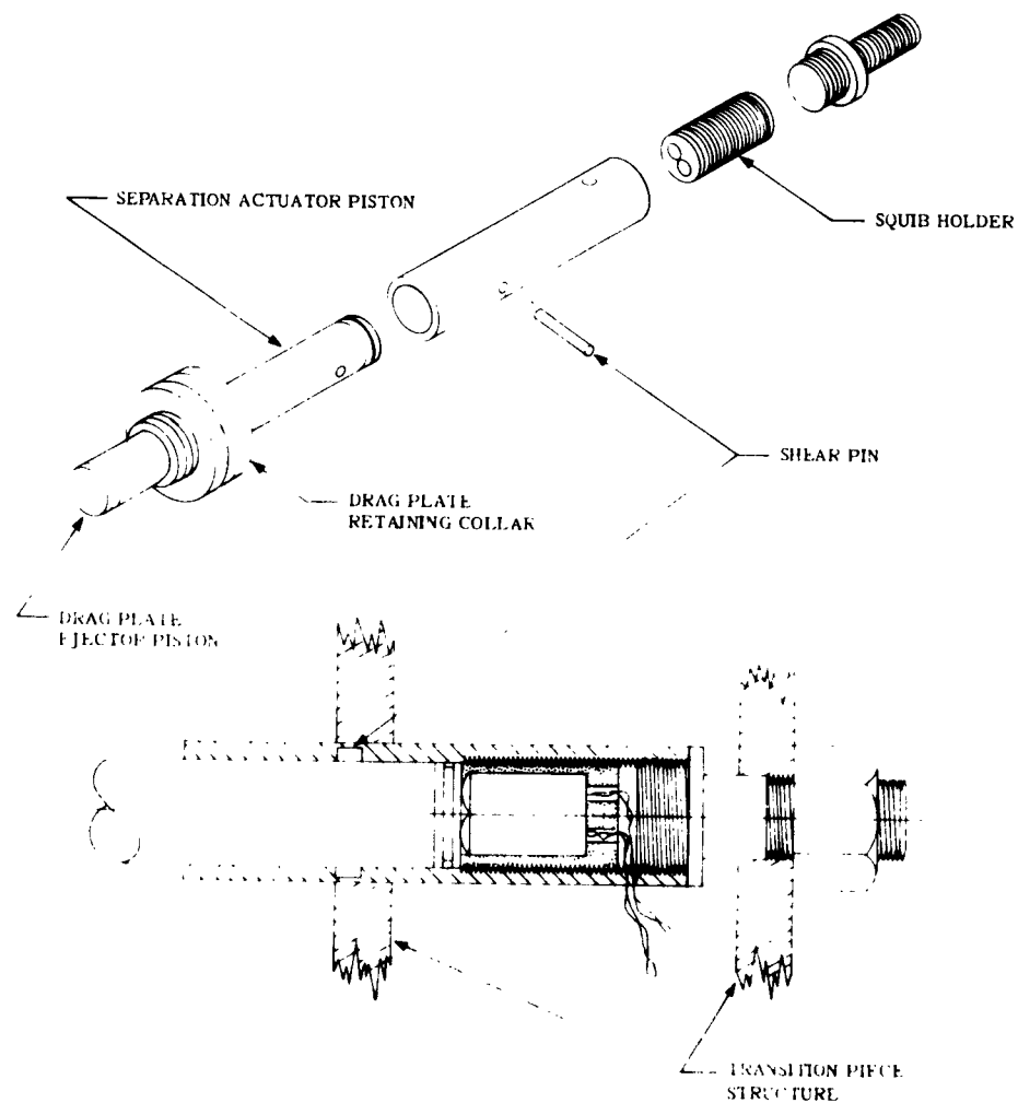
Figure 10. Payload Actuator.
