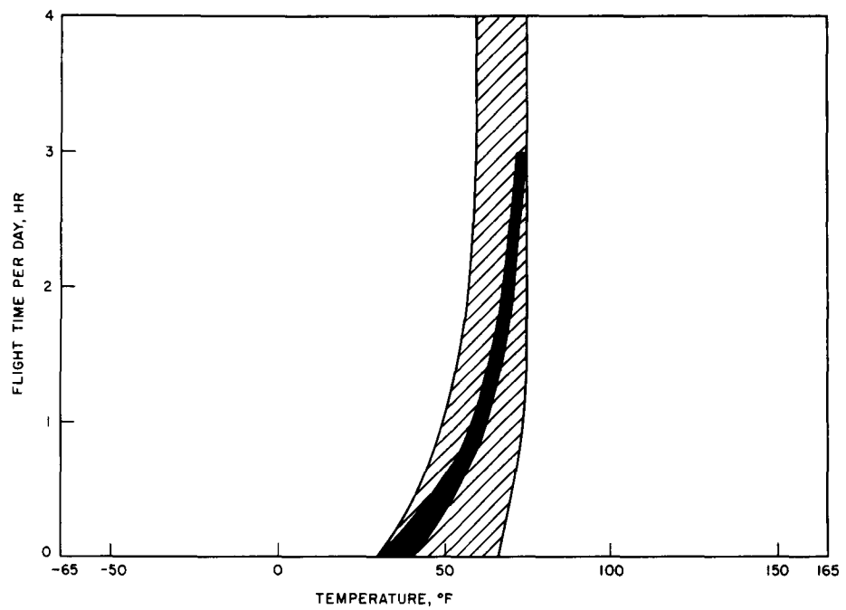
(a) Winter temperature spread. Solid section represents coldest day.
