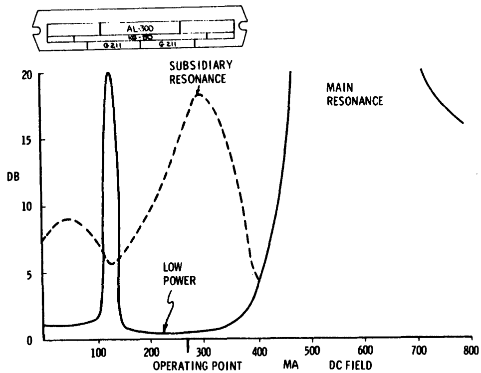
Figure 6. Electrical Characteristics of the Coaxial Subsidiary Resonance Limiter at 5.6 Gc
