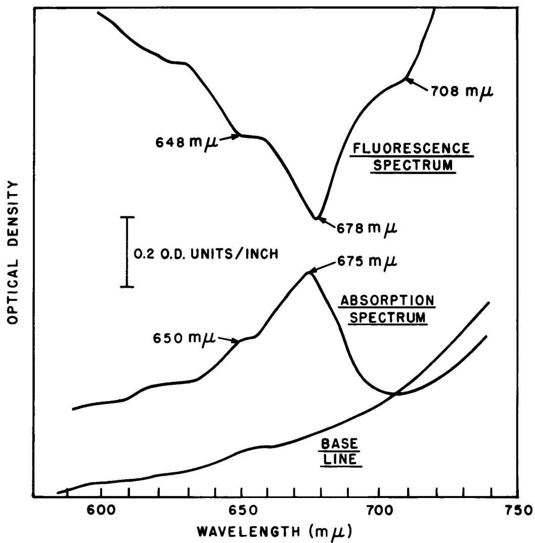
Figure 4 LOW TEMPERATURE ( -196^{\circ}\text{C} ) ABSORPTION AND FLUORESCENCE SPECTRA OF AQUEOUS SUSPENSIONS OF \text{CF}_{20-50}
