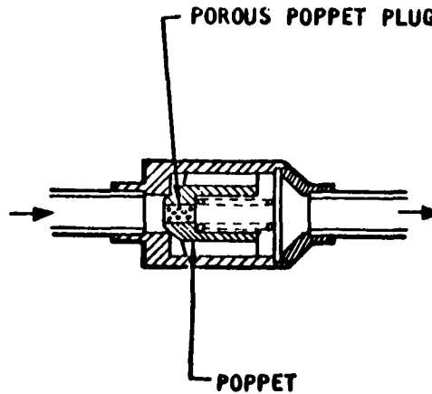
Figure 5. Vent Line Check Valve with Porous Plug
