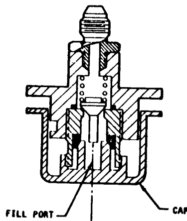
Figure 7. Fill Valve
