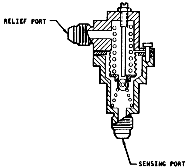
Figure 6. Regulated Pressure or System Pressure Relief Valve
