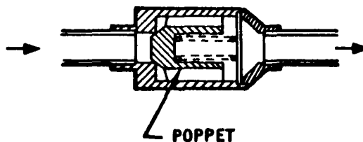
Figure 4. Fill Line Check Valve
