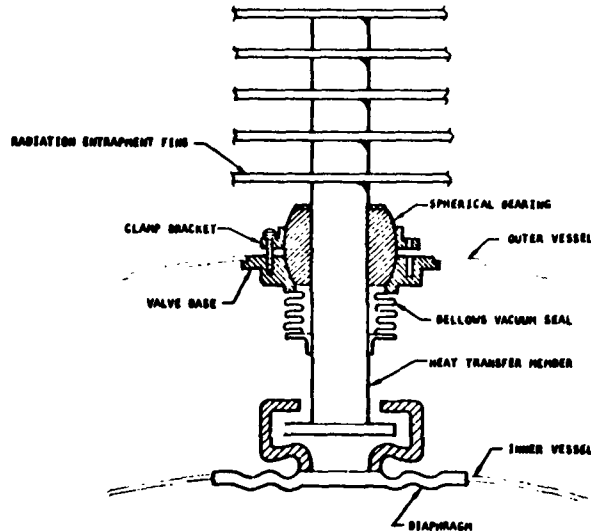
Figure 2. Thermal Shorting Valve
