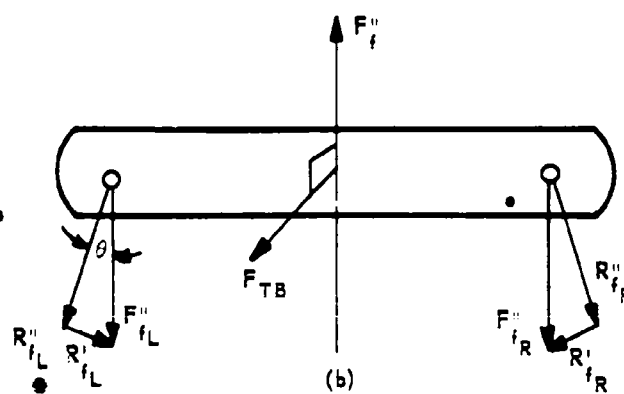
Fig 1 Bipod assembly (a) and yoke assembly (b)
