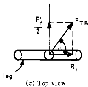
Fig 8 Bipod assembly
