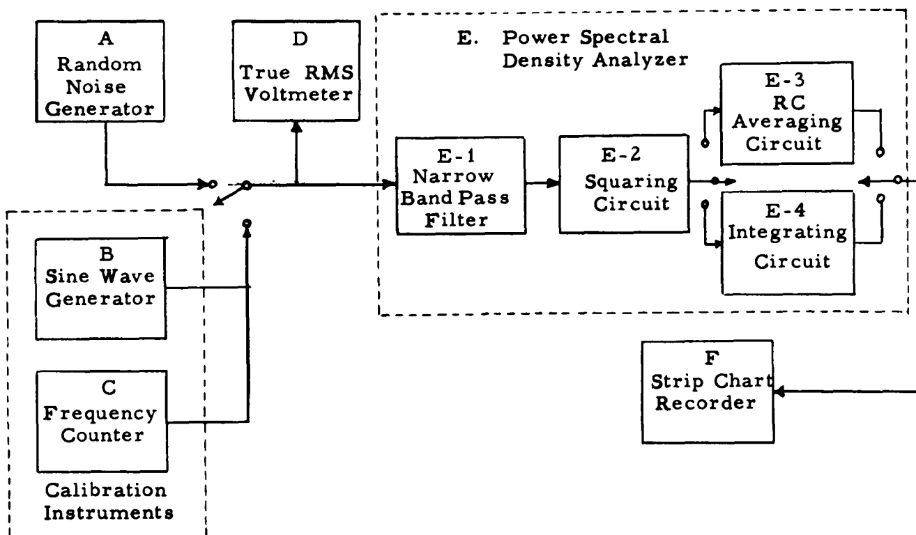
Figure 13.2 Block Diagram of Test Set-Up
