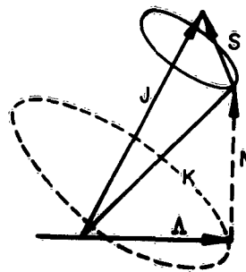
Fig. 4-2 Hund's Case "b"
