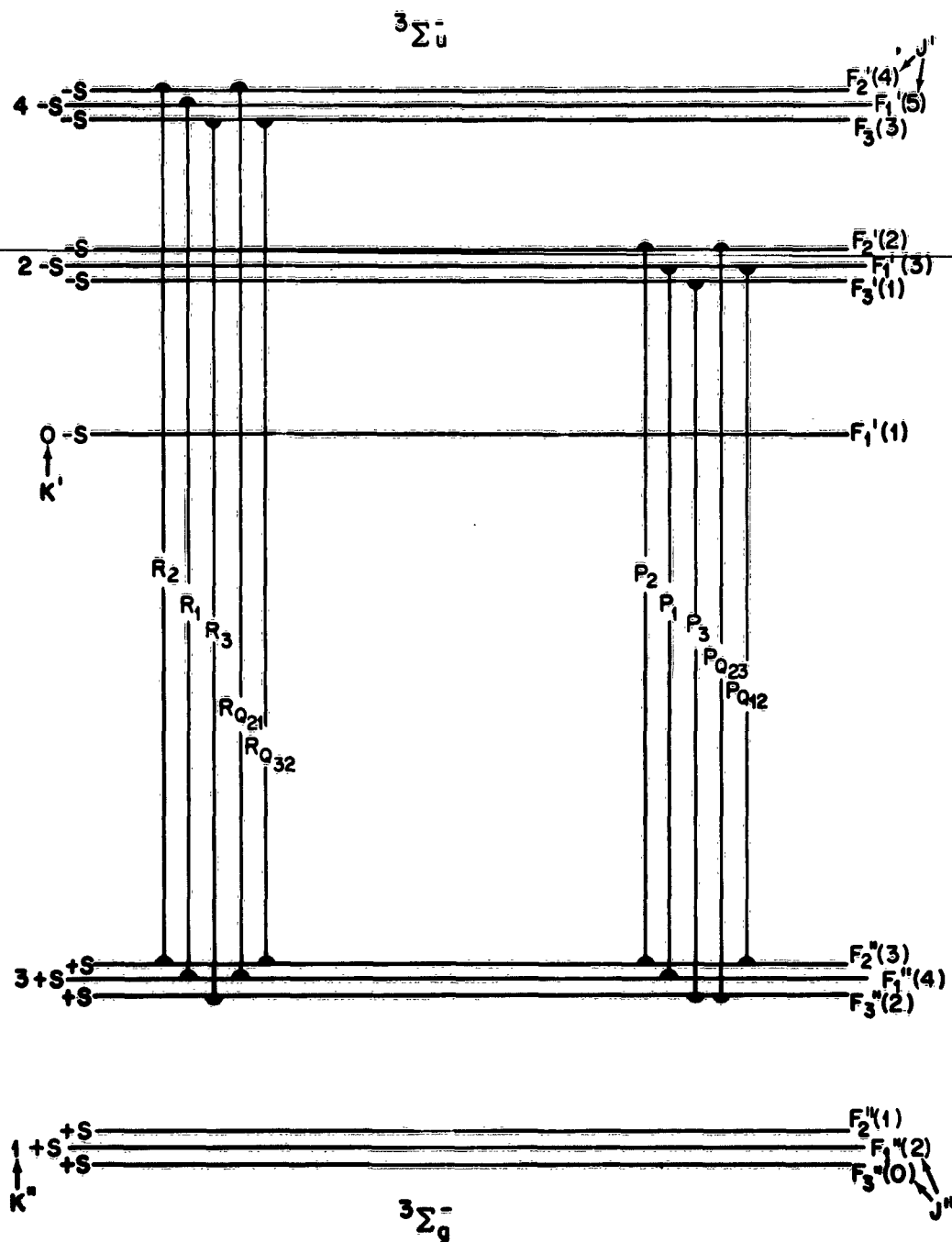
Fig. 4-3 B^3\Sigma_u^- - X^3\Sigma_g^- Band of O_2 (Schumann-Runge System)
