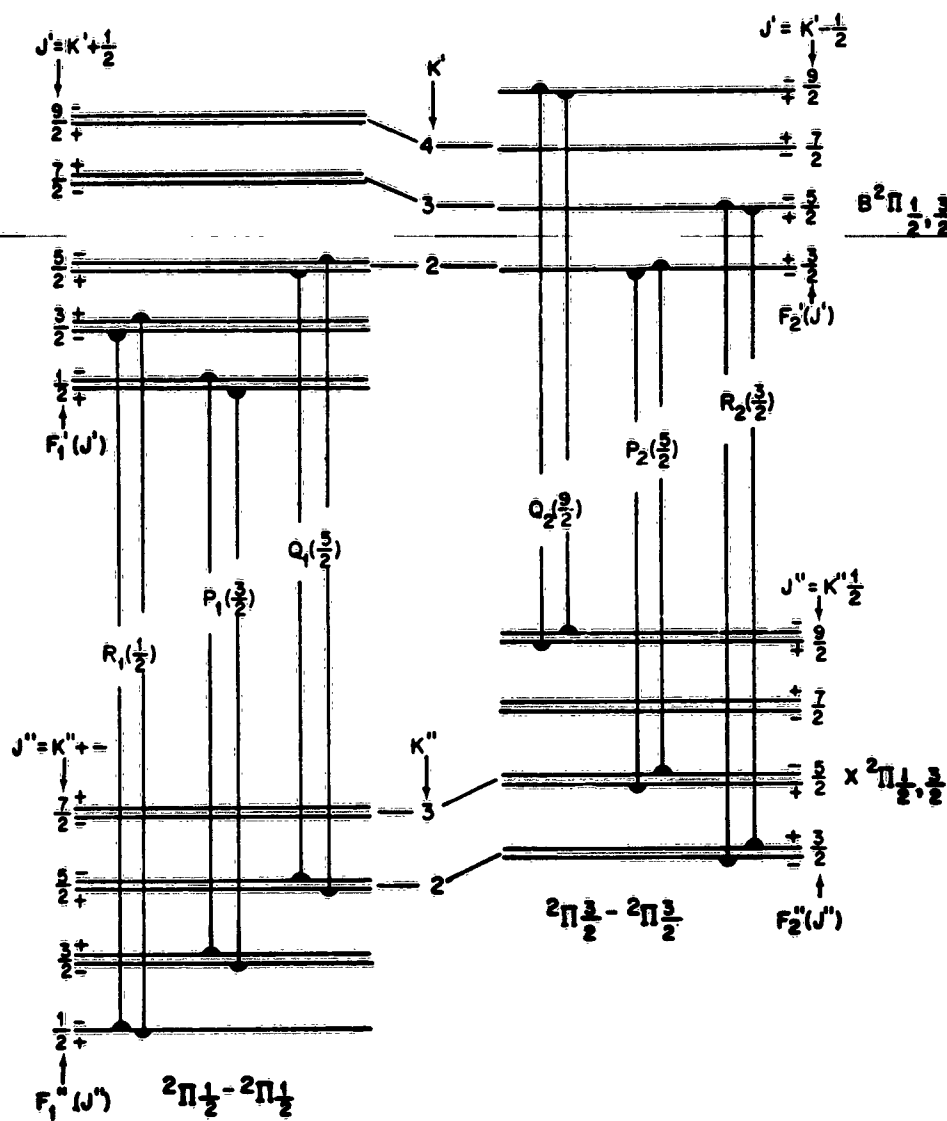
Fig. 4-7 B^2\Pi - X^2\Pi Band of NO ( \beta System)
