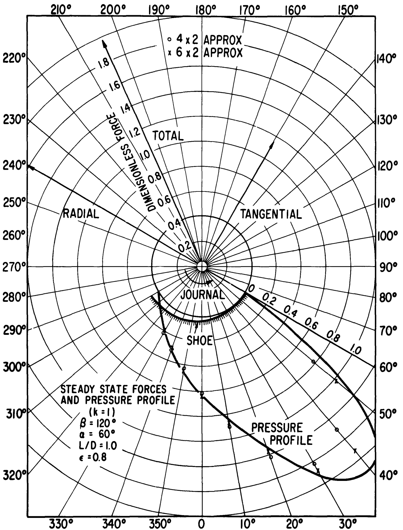
FIGURE I EXTRAPOLATED FORCES AND PRESSURE PROFILE
