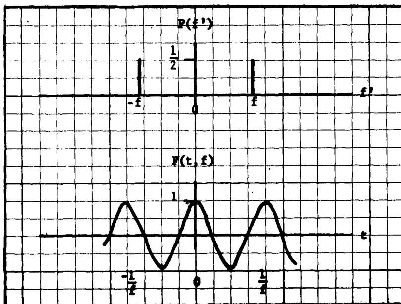
Fig. 9. The Fourier transform pair P(f', f) , F(t, f) for infinite variation of path difference.
