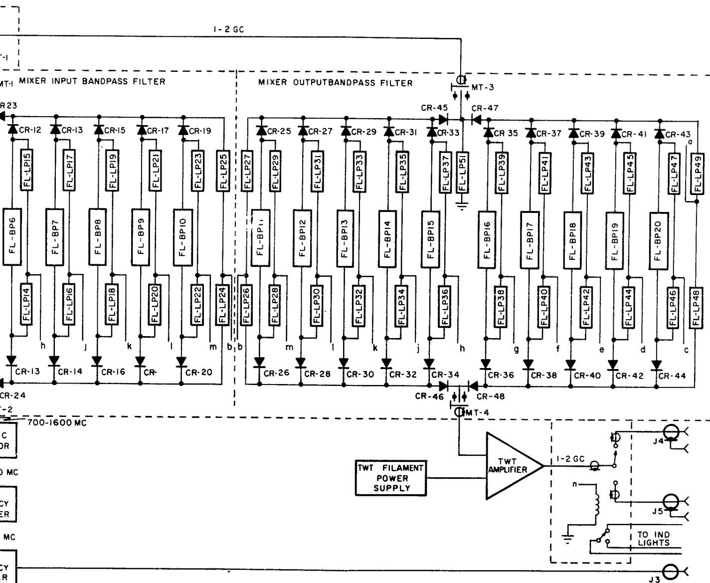
Figure 6-3. L-band frequency extender - block diagram
