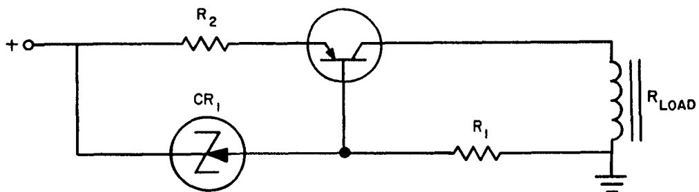
Figure 6-54. Alternate circuit configuration
