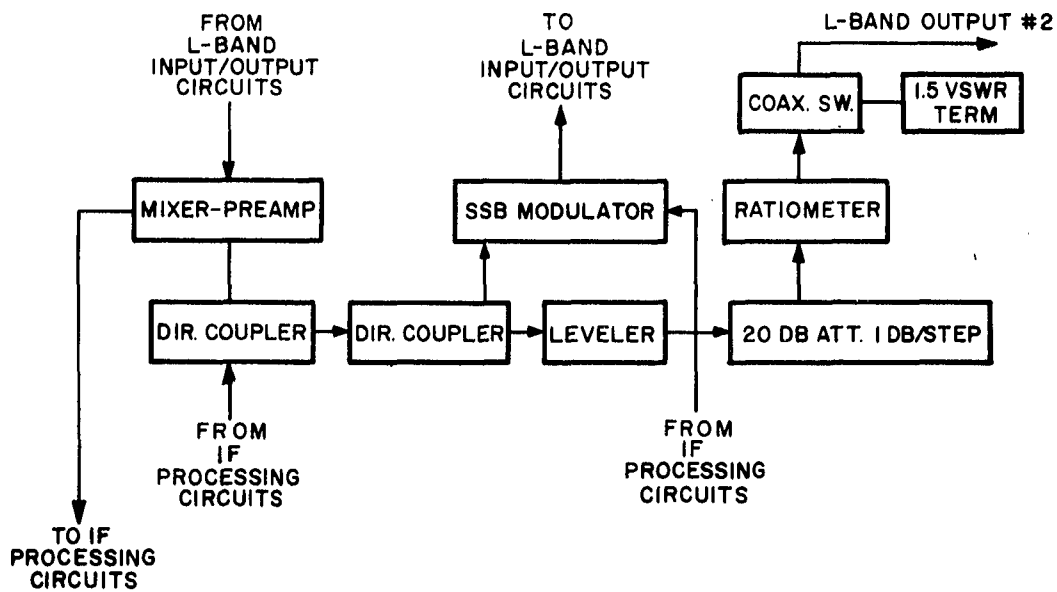
Figure 6-4. L-band conversion circuits - block diagram
