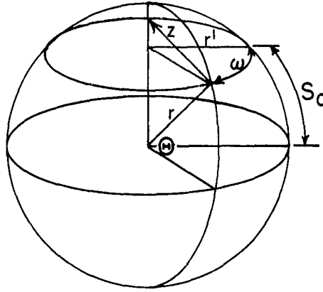
Figure 3. Diagram for Gore Width of Sphere
