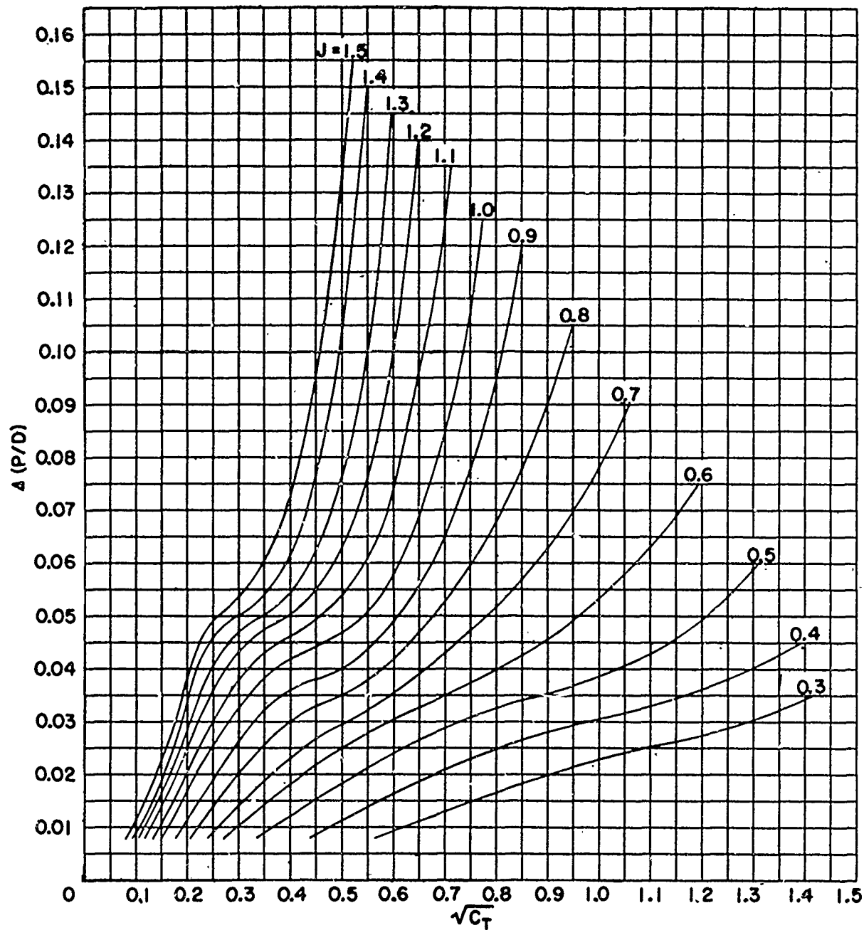
Figure 4e - Pitch Correction Coefficient \Delta(P/D) for Finite Cavitation Numbers for TMB 3-Bladed SC Propeller Series, EAR = 0.5
