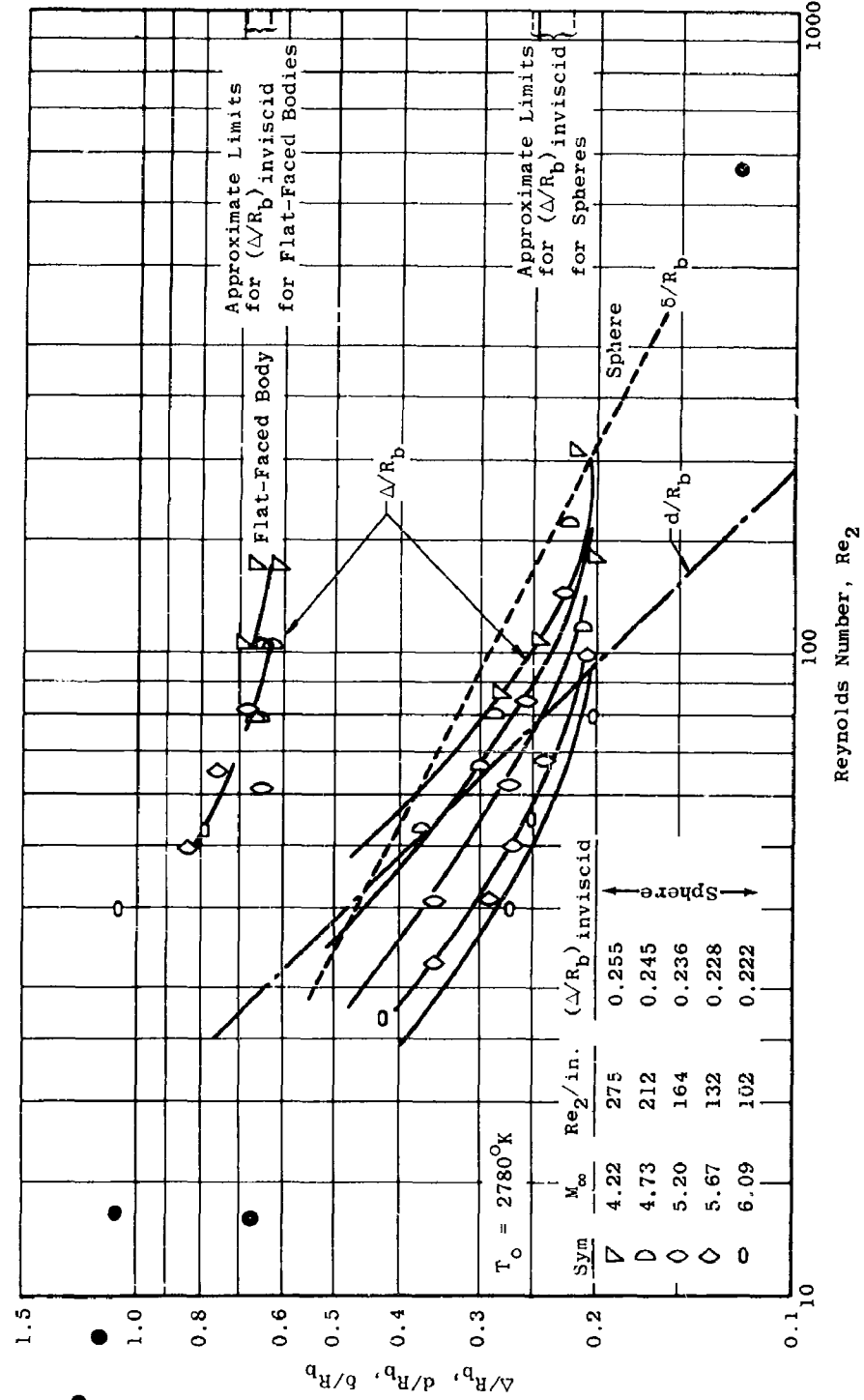
Fig. 3 Stagnation Region Shock Detachment Distance for a Water-Cooled Sphere and Flat-Faced Body in Argon ( T_w/T_o \approx 0.11 )
