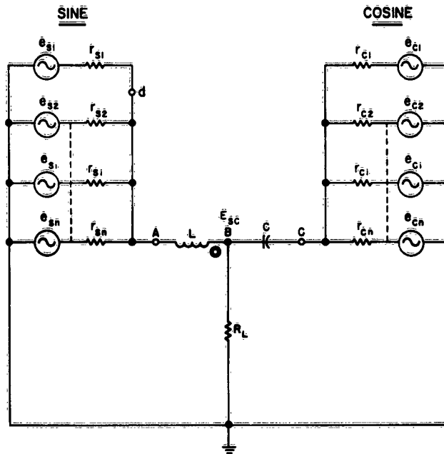
Figure A-1. Equivalent circuit No. 1.
