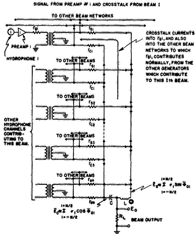
Figure B-1. Illustration of cross talk, showing the manner in which the summed beam quadrature voltages ( \bar{E}_s , \bar{E}_c ) can be considered single generators contributing cross-talk voltage to adjacent beams by means of inducing current flow back through a given generator (preamp) resistance.
