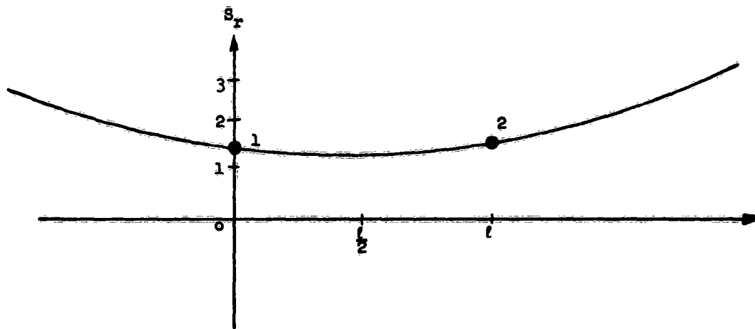
Fig. 16. Variation of the standard error of a corrected deviation. s_0 = 1 .
