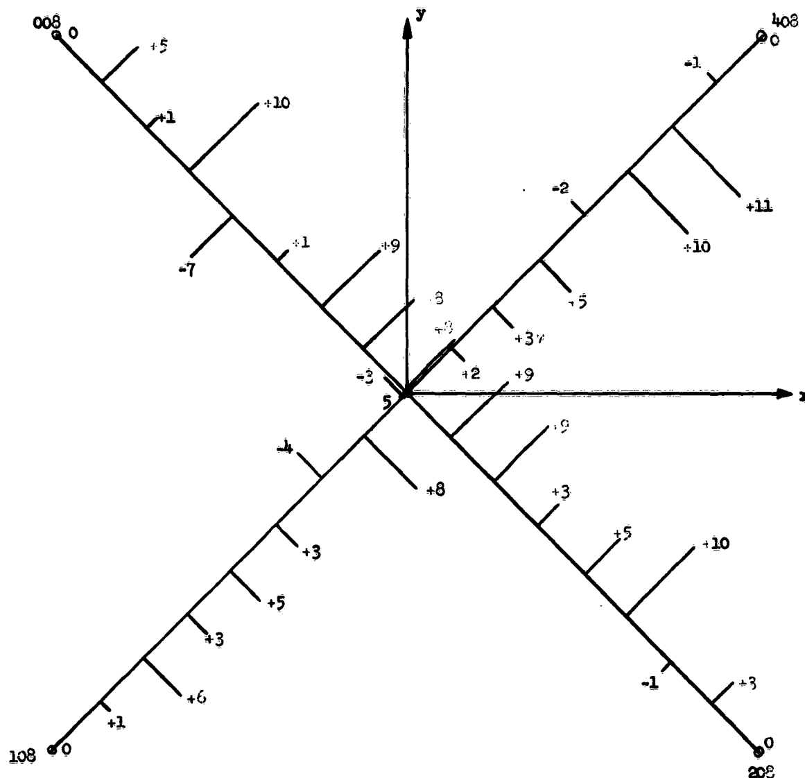
Fig. 19. Residuals along the diagonals, and orthogonal to the diagonals, after adjustment and after making the residuals zero in the points 108-408, 208-308 through translations and rotations of the diagonals. All data in microns.
