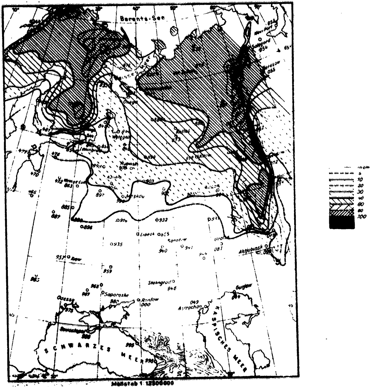
Map 18. Average depth of snow cover, 11-12 April
