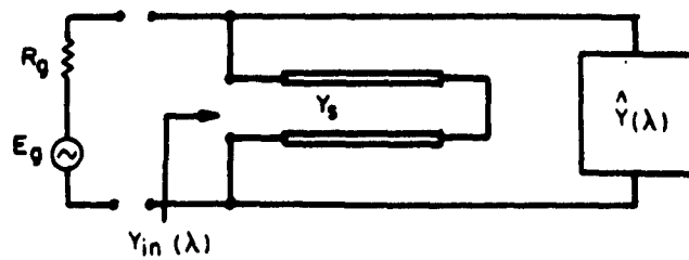
Fig. 14 Bandpass Filter Schematic
