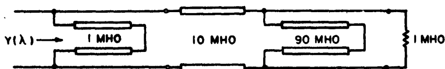
Figure 21 - Equivalent Network
