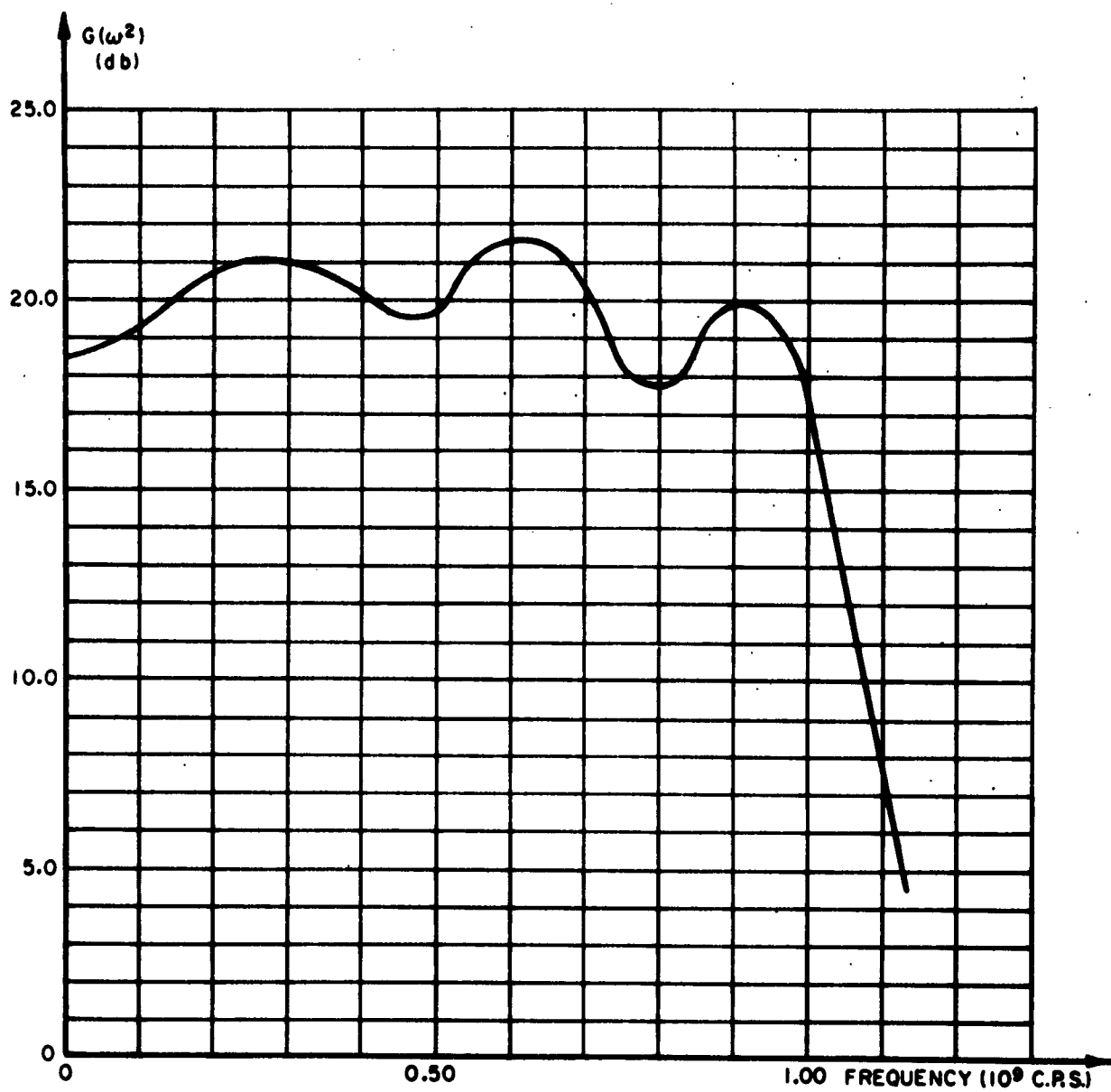
Fig. 29 Transducer Power Gain [G(\omega^2)] vs. Frequency
