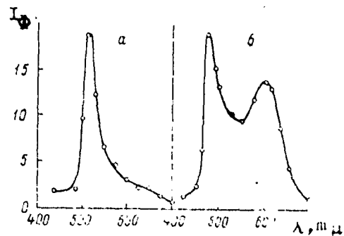
Fig. 16. Influence of annealing and tempering on the spectral distribution of the photocurrent in CdS single crystals. Photoconductivity spectrum after annealing: a - annealing; b - tempering.
