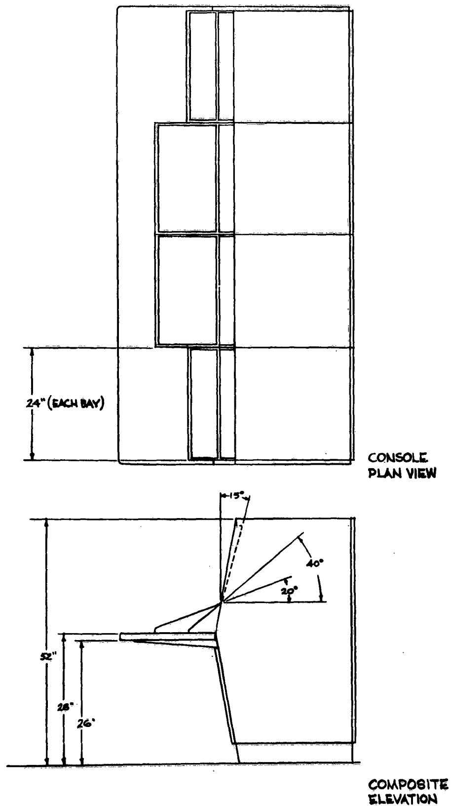
Fig. 4-3 Console Plan View and Composite Elevations
