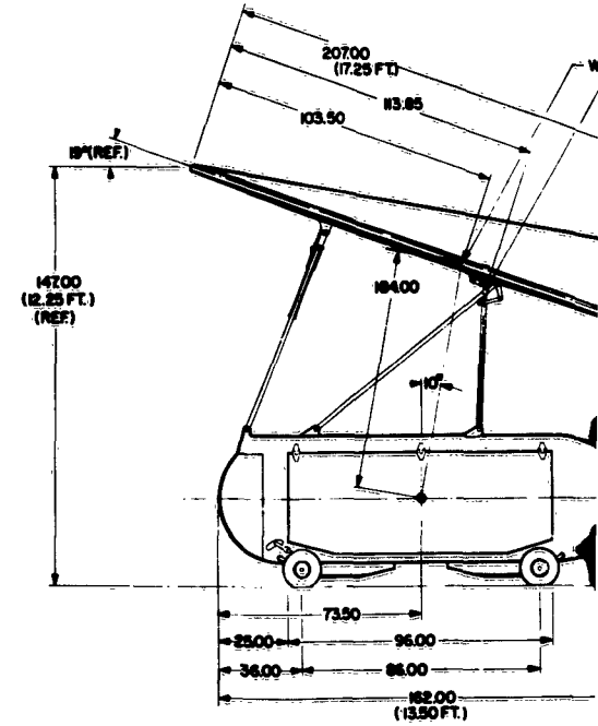
Dwg. 2 - B063-0013 General Arrangement - 1000 Lb. Flexible Wing Ca
