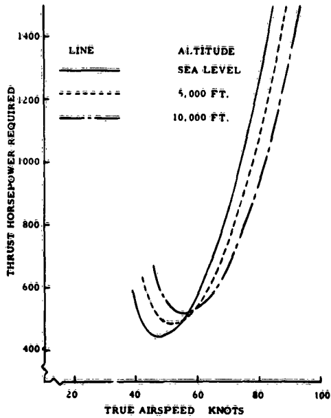
THRUST HORSEPOWER REQUIRED VS TRUE AIRSPEED ON STD. DAY 8000 LB PAYLOAD GLIDER W/S - 6.0 LB/FT 2
