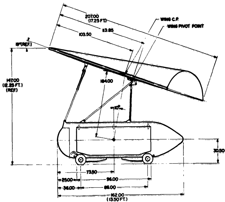
Dwg. 2 - B063-0013 General Arrangement - 1000 Lb. Flexible Wing Cargo Glider
