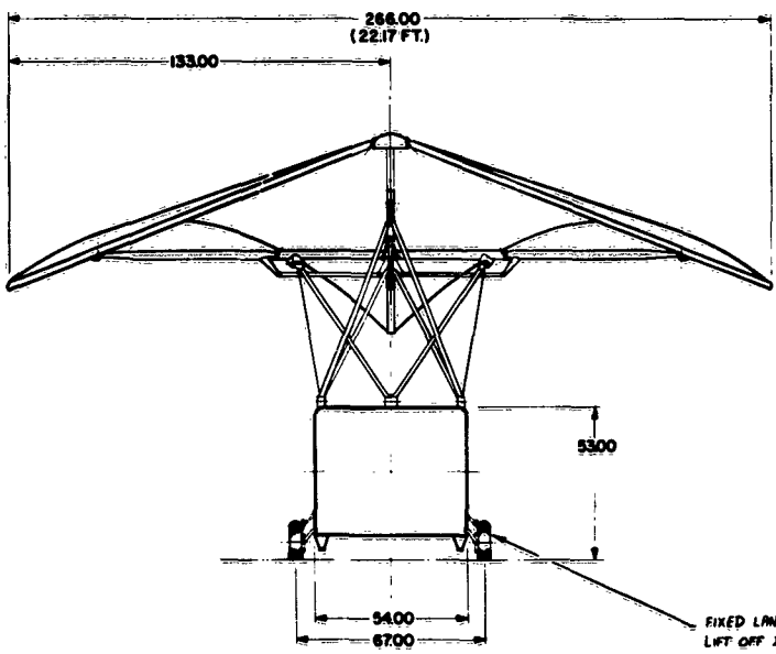
Dwg. 2 - B063-0013 General Arrangement - 1000 Lb. Flexible Wing Ca
