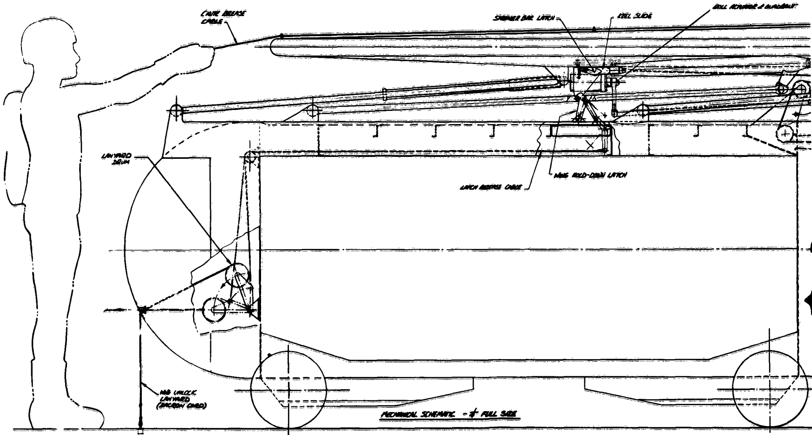
PHASE 3 - AIRS WALKER LAUNCHES CHAIR INTO AIR AND RELEASES LAUNCH BEAMS FREE FROM DOWN SLIDE SUPPORTS FROM AIRCRAFT & BARRIAGES
