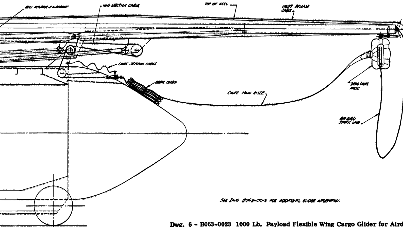
STAGE 5. CHUTE PACK FALLS FROM AFT END OF KEEL, RATE OF WING SPREAD LIMITED BY DESENSITIVE AIRFLOW BRANGS TO PREVENT EXCESSIVE AIR-STRUCTURE LOADS; KEEL SLAM LOCKS; DRAG CHUTE JETTISON.
