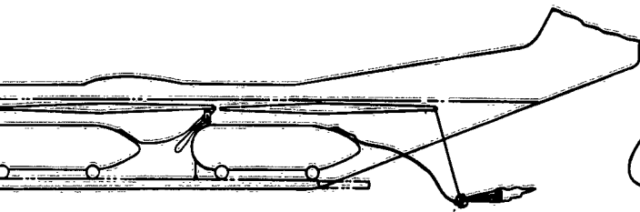
PHASE 2. CHUTE PACK FALLS FROM AFT END OF KEEL RP CHUTE STATIC LINE DEPLOYS CHUTE
