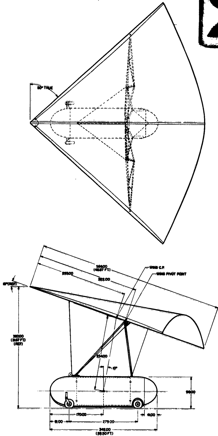
Dwg. 5 - B063-0018 General Arrangement - 8000 Lb.
