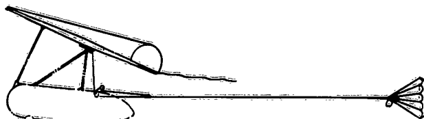
STAGE 5. CHUTE PACK FALLS FROM AFT END OF KEEL, RATE OF WING SPREAD LIMITED BY DESENSITIVE AIRFLOW BRANGS TO PREVENT EXCESSIVE AIR-STRUCTURE LOADS; KEEL SLAM LOCKS; DRAG CHUTE JETTISON.
