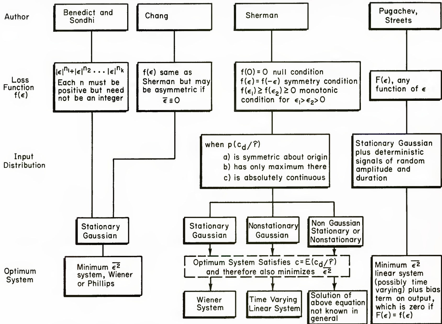
Figure 7. Summary of Minimum \bar{f}(\epsilon) Systems
