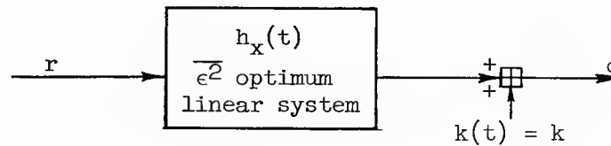
Figure 9. Pugachev's Optimum System
