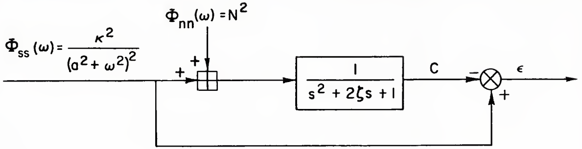
Figure 17. System for Investigation of Error Exceedances
