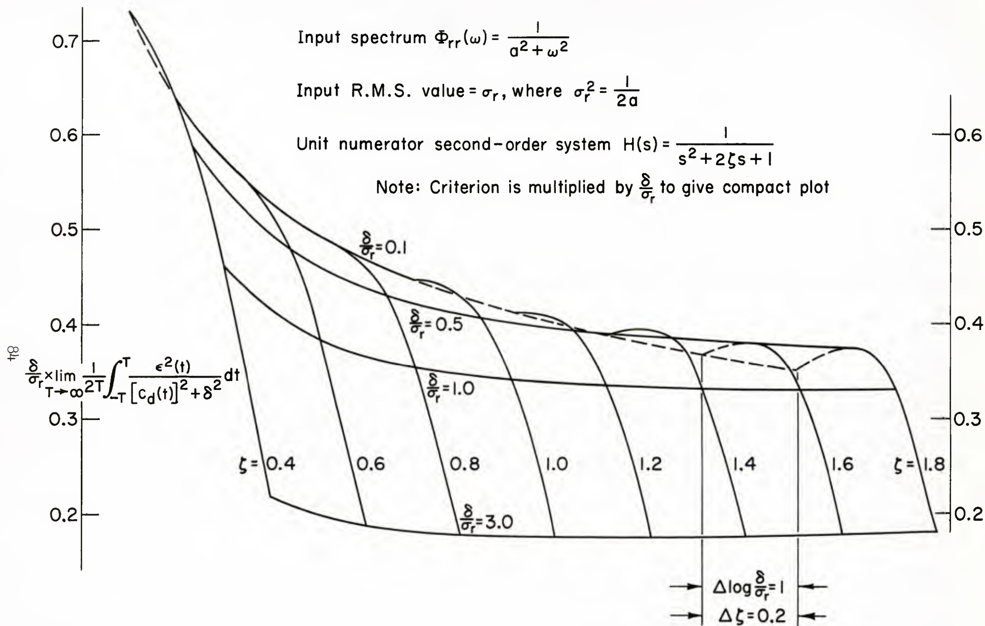
Figure 22. \frac{\delta}{\sigma_r} \times Glover's Criterion: Carpet of \frac{\delta}{\sigma_r} \lim_{T \rightarrow \infty} \frac{1}{2T} \int_{-T}^{+T} \frac{\epsilon^2(t)}{[c_d(t)]^2 + \delta^2} dt vs \zeta and \frac{\delta}{\sigma_r}
