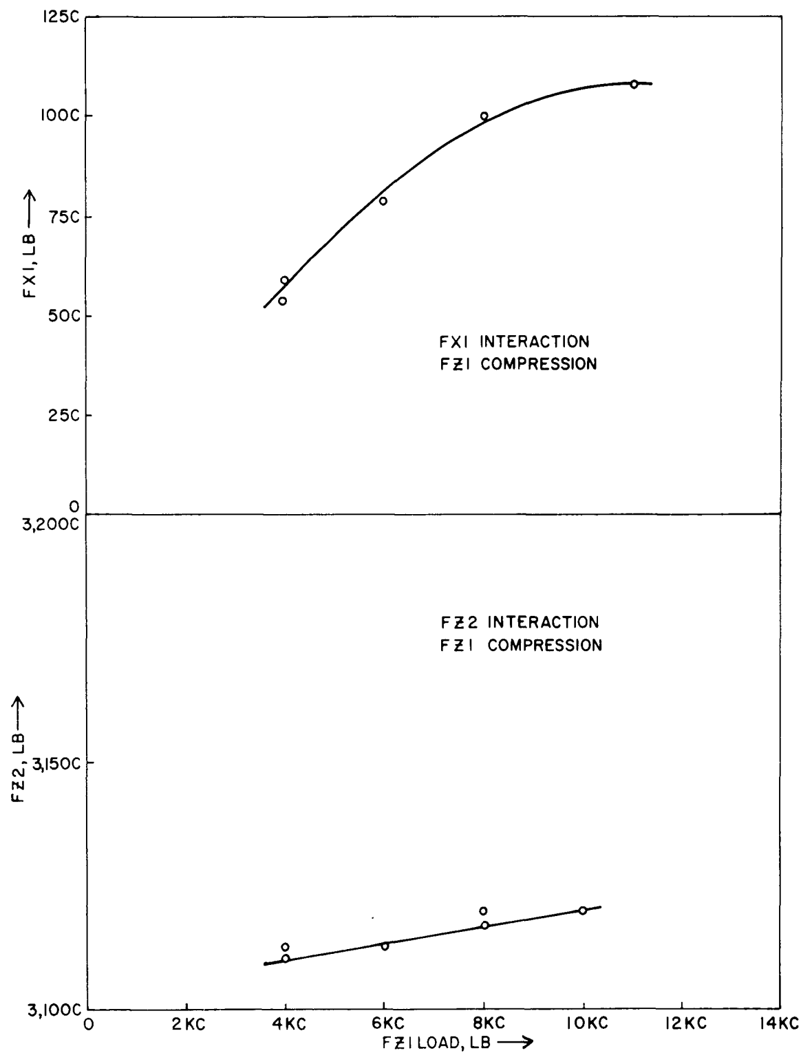
FIG. 9. Calibration Curves of Interaction Forces. Top, FX1 interaction, FZ1 compression; bottom, FZ2 interaction, FZ1 compression.
