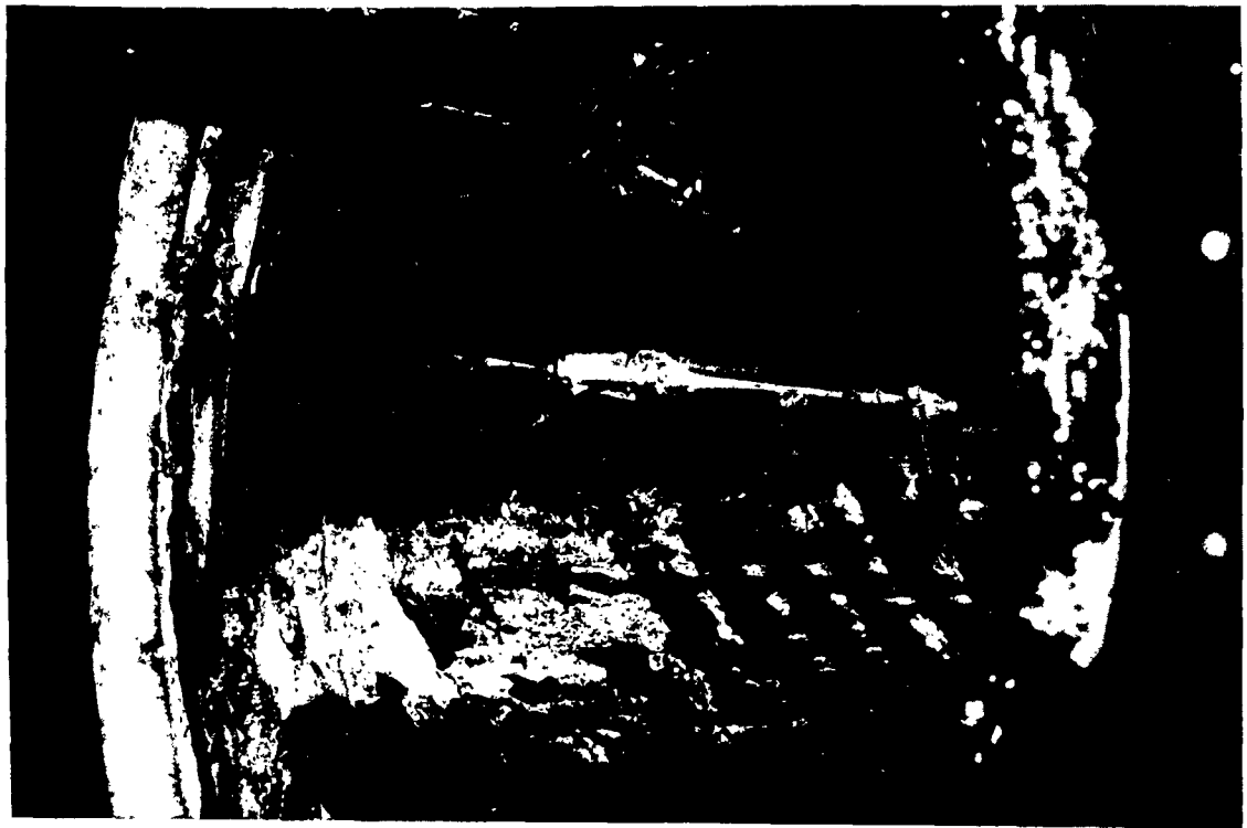
FIG. 55. Entrance Section Burnout of Stainless Steel Diffuser Liner.
