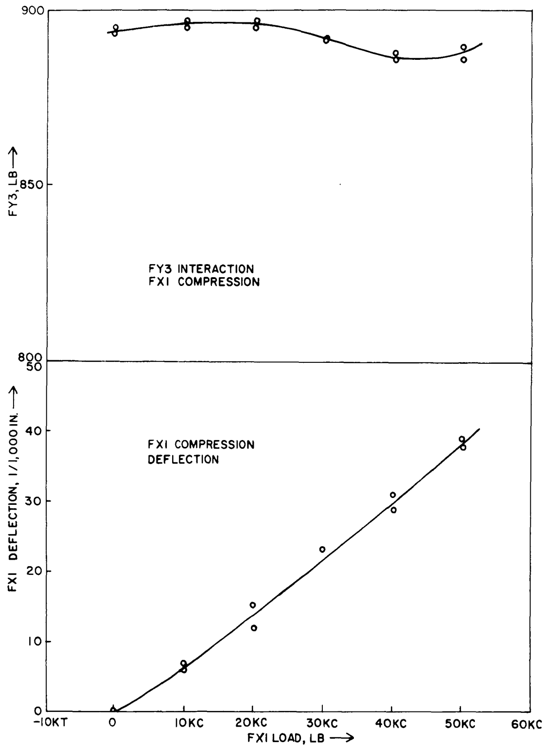
FIG. 8. Calibration Curves of Interaction Forces. Top, FY3 interaction, FX1 compression; bottom, FX1 compression, deflection.
