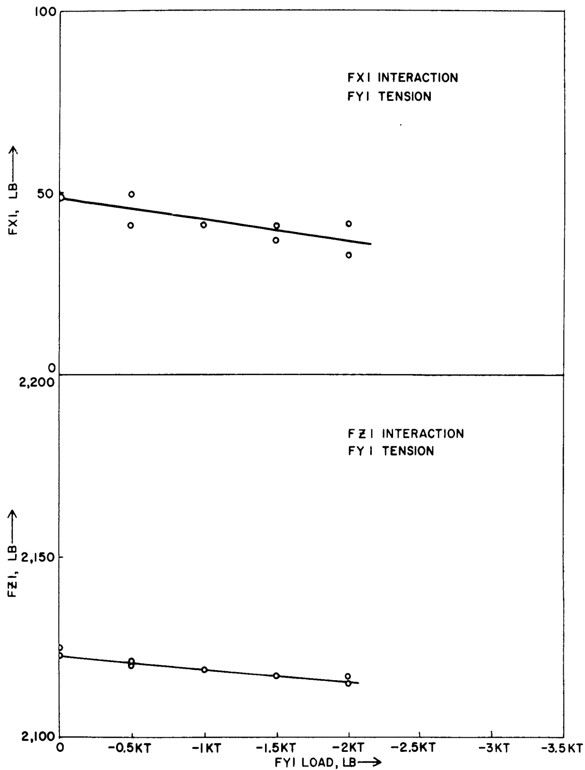
FIG. 24. Calibration Curves of Interaction Forces. Top, FXI interaction, FYI tension; bottom, FZI interaction, FYI tension.
