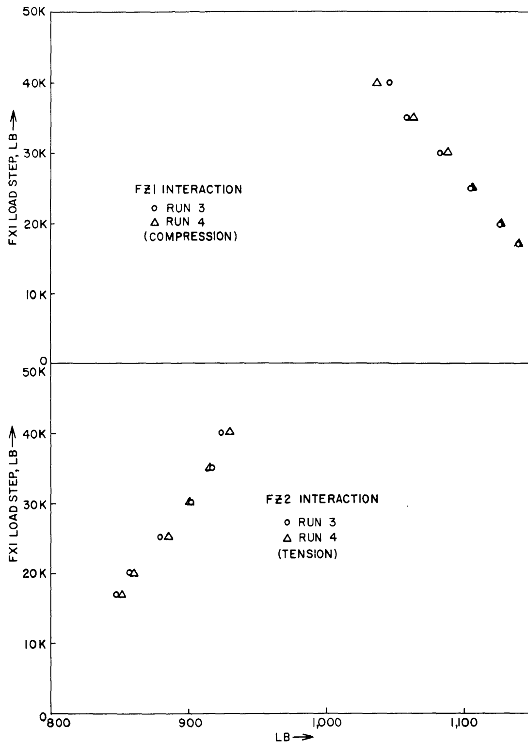
FIG. 45. Vertical Load Interaction Data.
