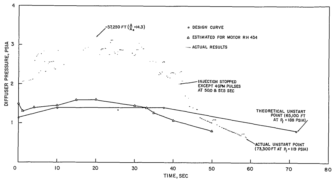
FIG. 56. Diffuser Performance, ST-60.
