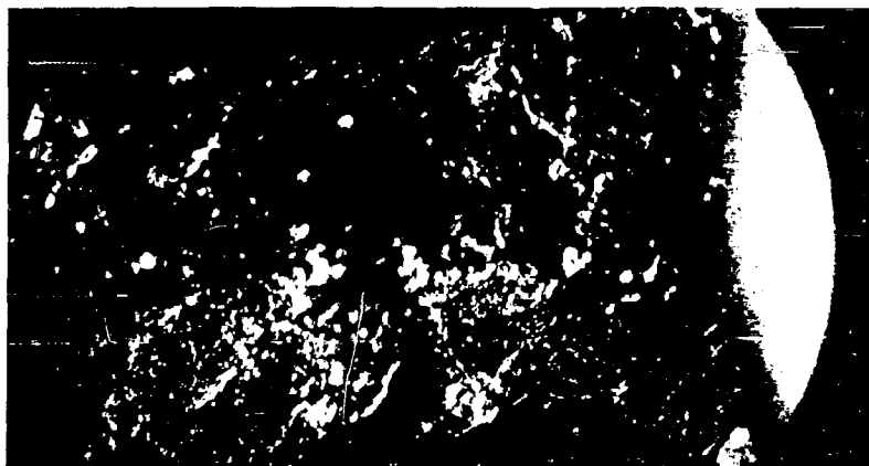
FIGURE 12C. CROSS SECTION OF TUNGSTEN CARBIDE SPECIMEN W-F AFTER 3.54% WEIGHT LOSS. NO WC VISIBLE. MAGNIFICATION 50X. POLARIZED LIGHT.
