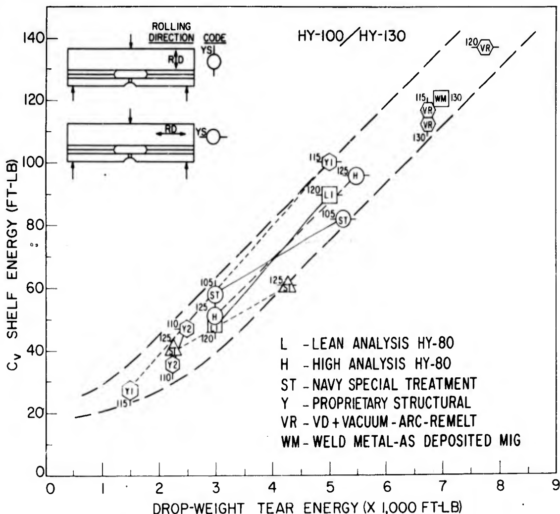
Fig. 22 - Illustrating the wide range of DWTT energy values developed by various steels of the 100 to 130 ksi yield strength range
