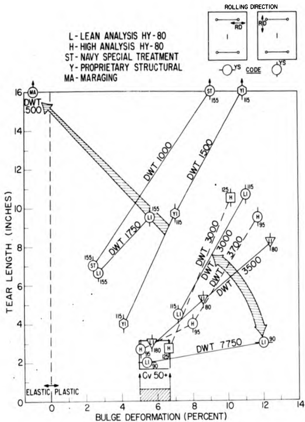
Fig. 18 - Explosion tear test data, previously presented in Fig. 15, referenced to the drop-weight tear test energy adsorption for tests conducted at the same (30°F) temperature as used for the explosion test
