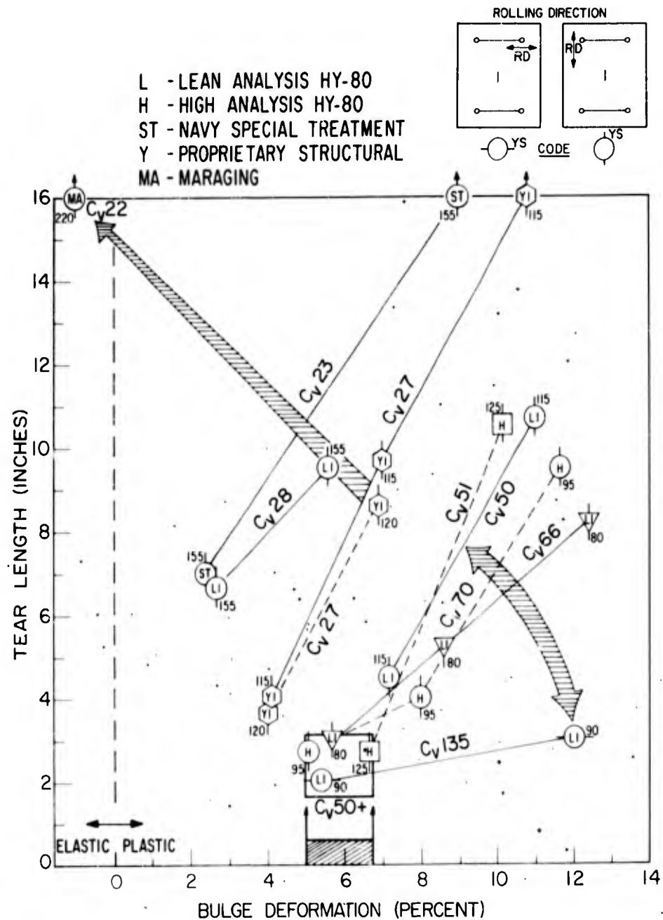
Fig. 15 - Total tear length (summation of the two ends of tear extensions) resulting from explosion loading to various levels of bulge deformation - C_v -SE of the steels are indicated. The connecting lines indicate tests of different plates of the same steel loaded to the indicated levels of deformation.
