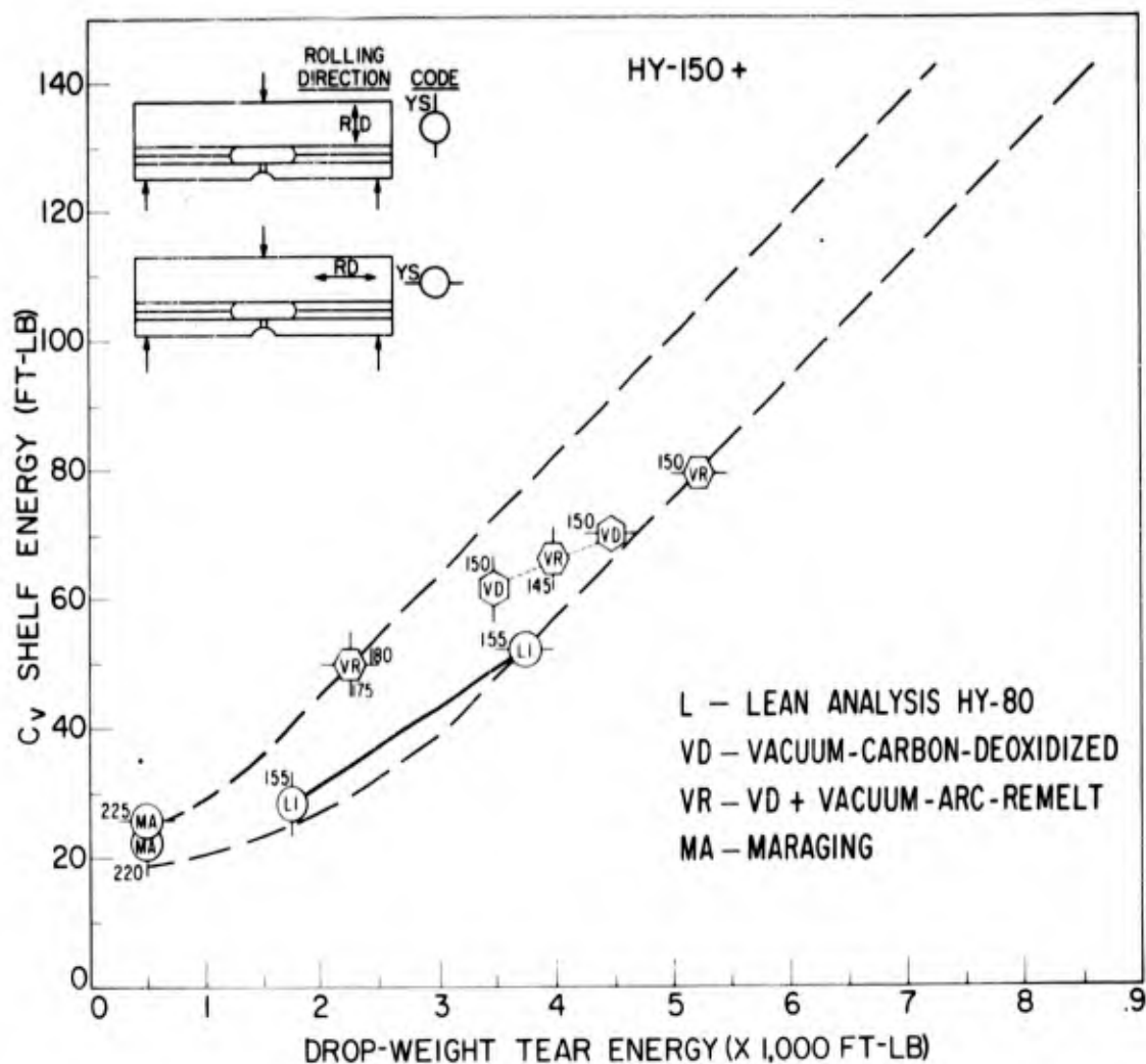
Fig. 23 - Illustrating the range of DWTT energy values developed by various Q&T steels of the 150 to 180 ksi yield strength range. Values obtained for the 220 to 225ksi yield strength Maraging steels are provided for comparison.
