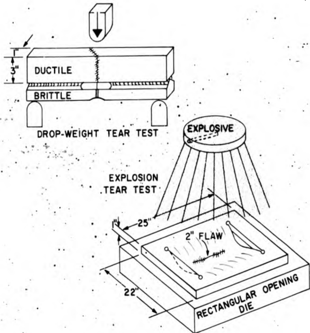
Fig. 12 - Features of drop-weight tear and explosion tear tests
