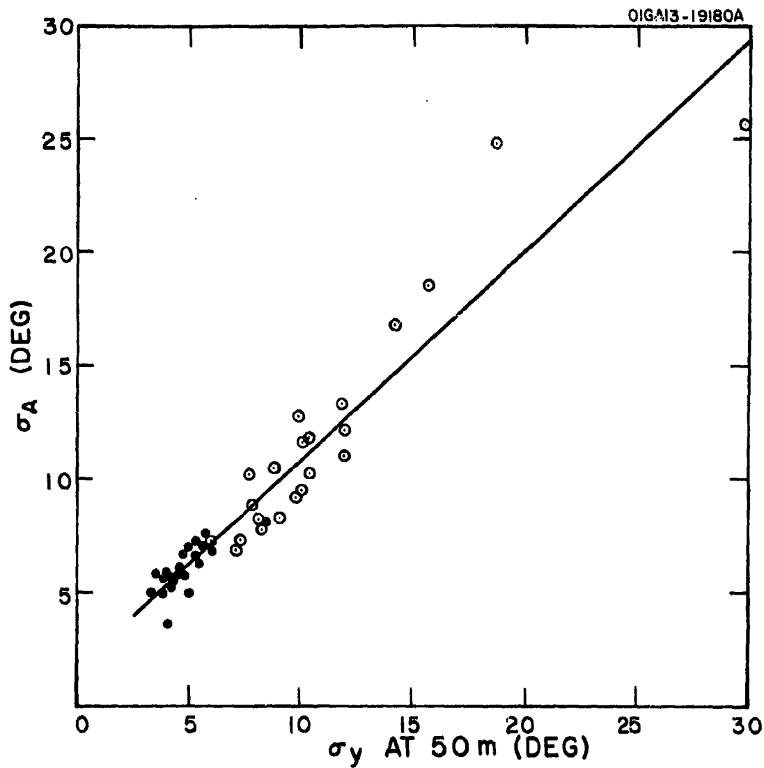
Figure 10. Standard deviation of azimuth wind direction versus the crosswind standard deviation of concentration at 50 m for Prairie Grass data. Daytime experiments are indicated by open circles and nighttime experiments by filled circles.
