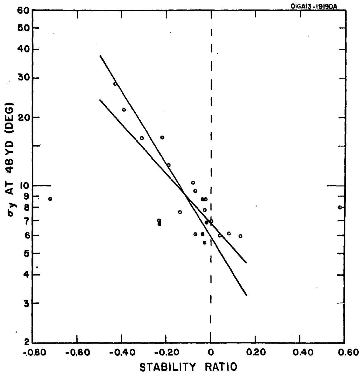
Figure 11. Crosswind standard deviation of concentration at 48 yd versus the Stability Ratio for the Dugway trials. Solid lines are least-squares regression lines; the two points beyond the limits of the regression lines were omitted in the analysis.
