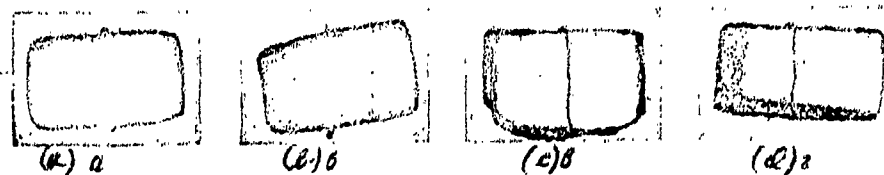
Figure 5. Specimens of steel #3 with different coatings, after heat resistance test at 1100^{\circ} : a - without spray coating, after 80 hours; b - NiCr coating, after 100 hours; c - NiCr + Al_2O_3 coating, after 100 hours; d - NiCr + Al_2O_3 coating and vacuum treatment, after 100 hours.
