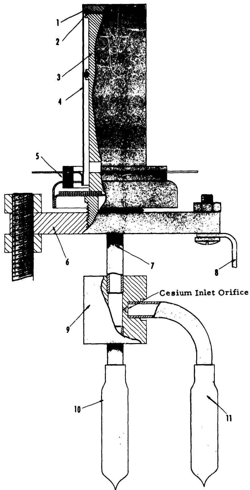
Figure 5. Corrosion Test Vehicle
