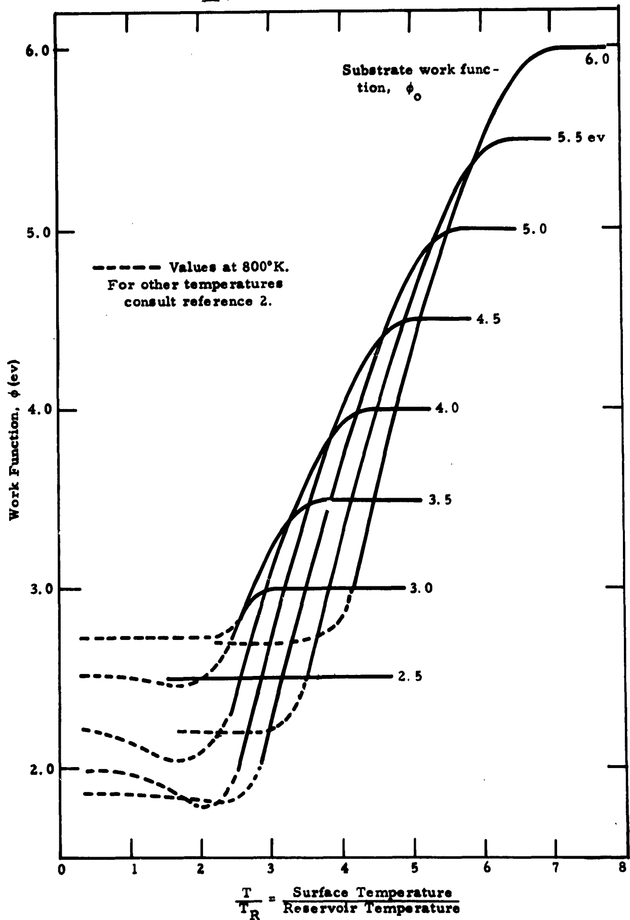
Figure 1. Work Function of Surface With Adsorbed Cesium
