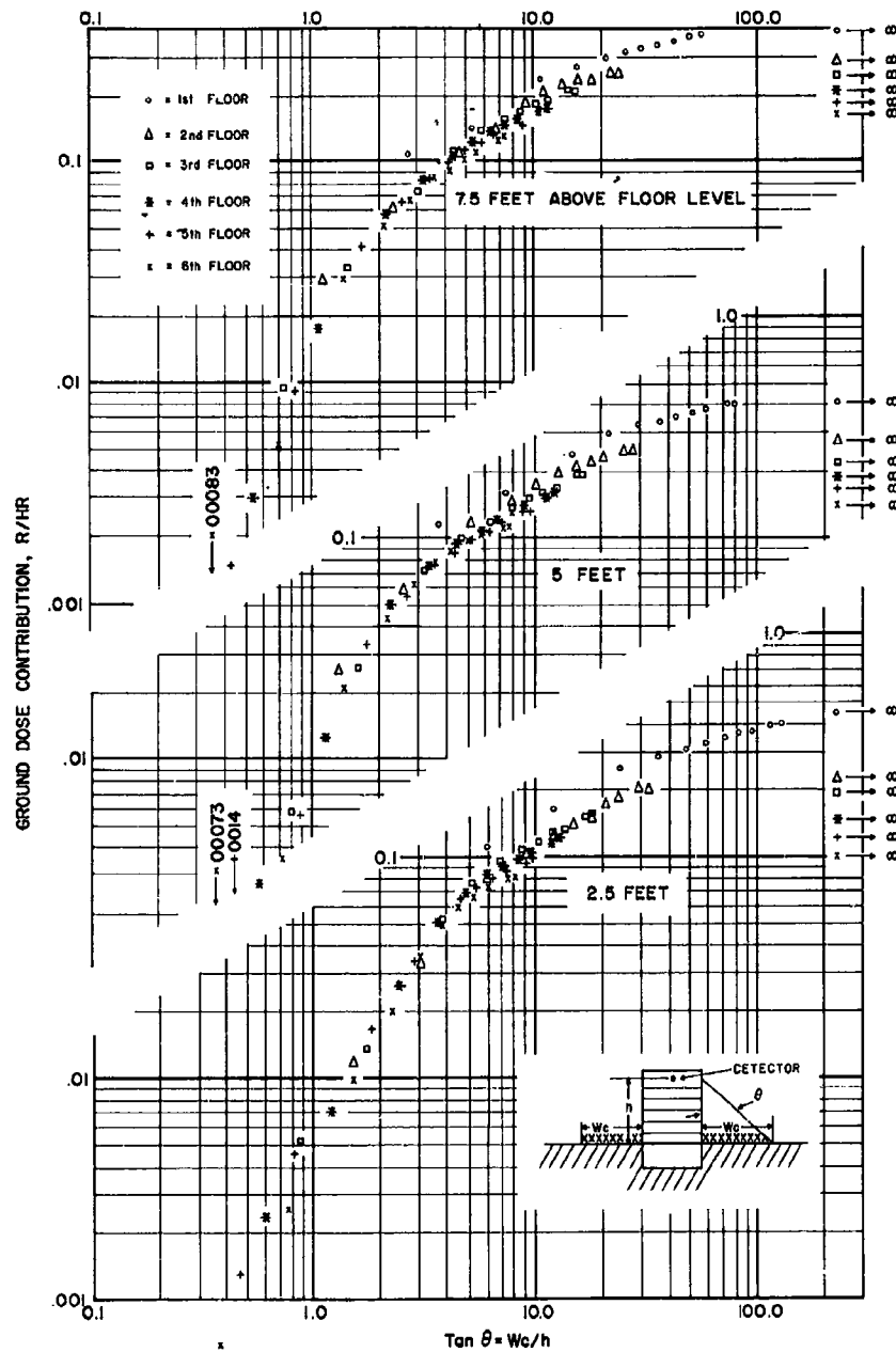
Figure 18. Full-Scale Dose Rate vs. W/h for Corner Position of Building with 20 psf Walls and 80 psf Floors
