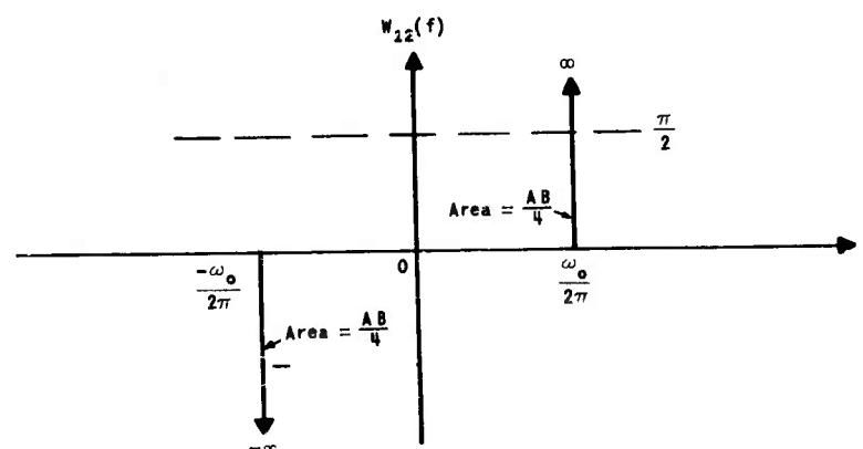
Figure A-6 - Plot of cross-power spectra W_{12}(f) of the periodic functions x_1(t) and x_2(t)
