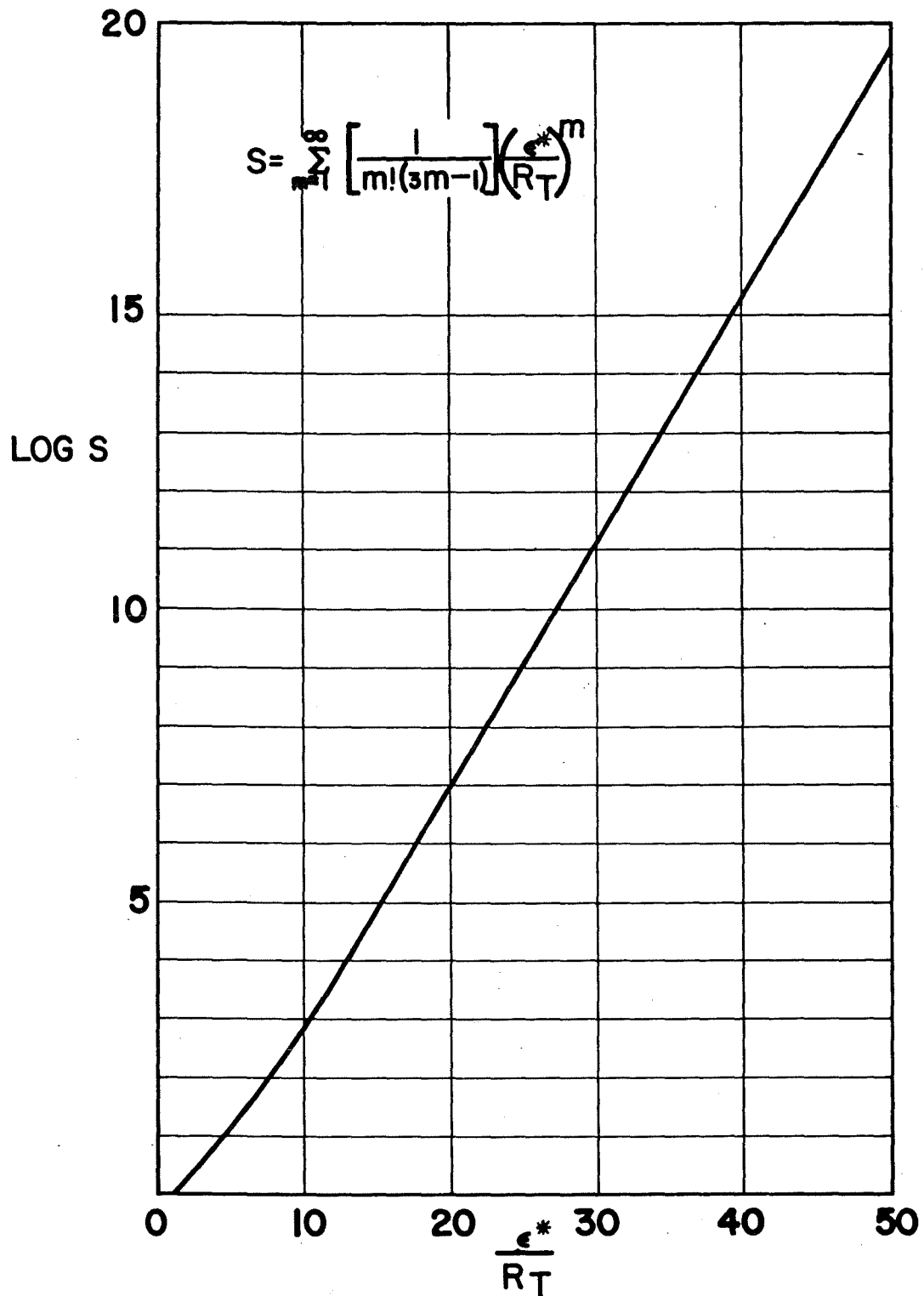
Fig. 2.2 Machine Computed Values of Gas-Solid Collision Sum
