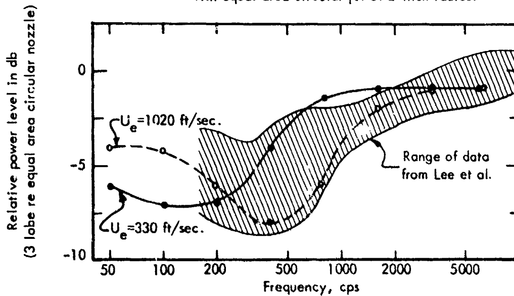
Figure 80. Comparison of acoustic power reduction calculated for three lobe 2.83 inch radius nozzle relative to 2 inch radius circular nozzle with data from Lee et al. for five pressure ratios
