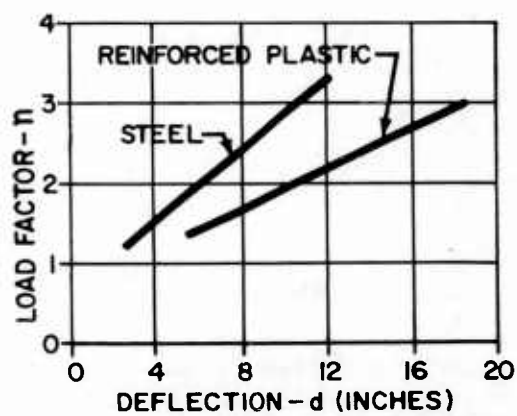
FIGURE 27. LOAD FACTOR VS. DEFLECTION L-19 LANDING GEAR
