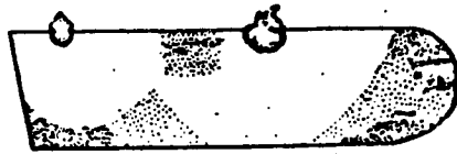
Fig. 9. Resistance of LM-5 coating to oxygen infiltration. Clear portions correspond to oxygen contaminated niobium. Corrosion by a mixture of hydrofluoric acid: nitric acid; glycerol = 1:1:2. Magnification 3X.
