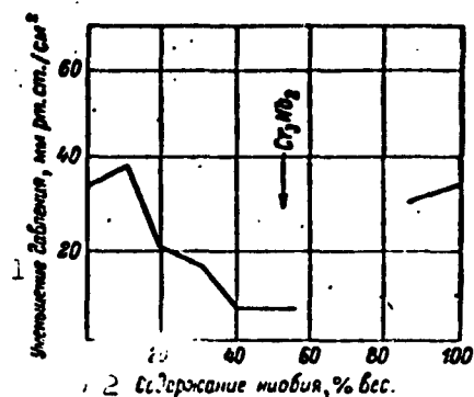
Fig. 7. Oxidation resistance of chromium-niobium alloys. Pressure drop in sealed vessel after heating over a period of 40 minutes [24].
