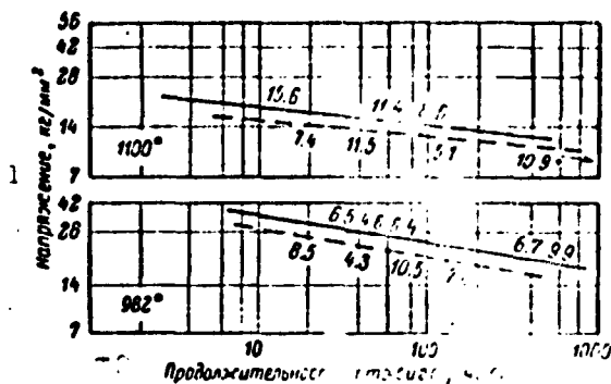
Fig. 1. Long-term strength of technical-grade niobium.
