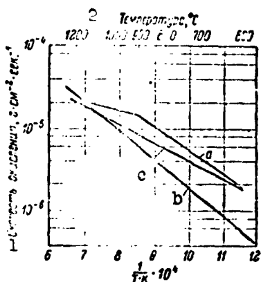
Fig. 2. Relationship of oxidation rate of niobium to temperature. a) In an atmosphere of dry air according to Inoya; b) in an atmosphere of dry air according to Klopp et al.; c) in an atmosphere of moist air [3, page 506]. 1) Oxidation rate, g cm -2 sec -1 ; 2) temperature, °C.
