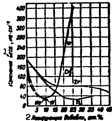
Fig. 15. Weight change of niobium alloys after heating at 1200° for 2 hours in air atmosphere [36]. 1) Weight change, \text{mg} \cdot \text{cm}^{-2} ; 2) alloying additives, atom-%.
