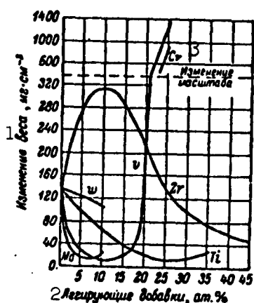
Fig. 14. Change in weight of niobium alloys after heating at 1000^{\circ} for 5 hours in an atmosphere of air [36].
