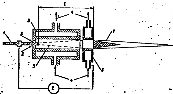
Fig. 12. Diagram of apparatus for production of ionized stream. 1) Rod electrode; 2) incoming gas; 3) channel; 4) cooling water; 5) trunk of arc; 6) ring-shaped electrode; 7) ionized stream; L is the distance the electrode is sunk; E is the power supply (33).
