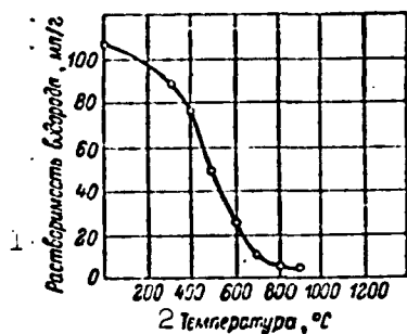
Fig. 3. Dependence of solubility of hydrogen in niobium upon temperature [14, page 135]. 1) Solubility of hydrogen, ml/g; 2) temperature, °C.
