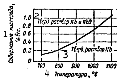
Fig. 4. Dependence of solubility of oxygen in niobium on temperature [15]. 1) Oxygen content, % by weight; 2) solid solution in Nb; and NbO; 3) solid solution in Nb; 4) temperature, °C.
