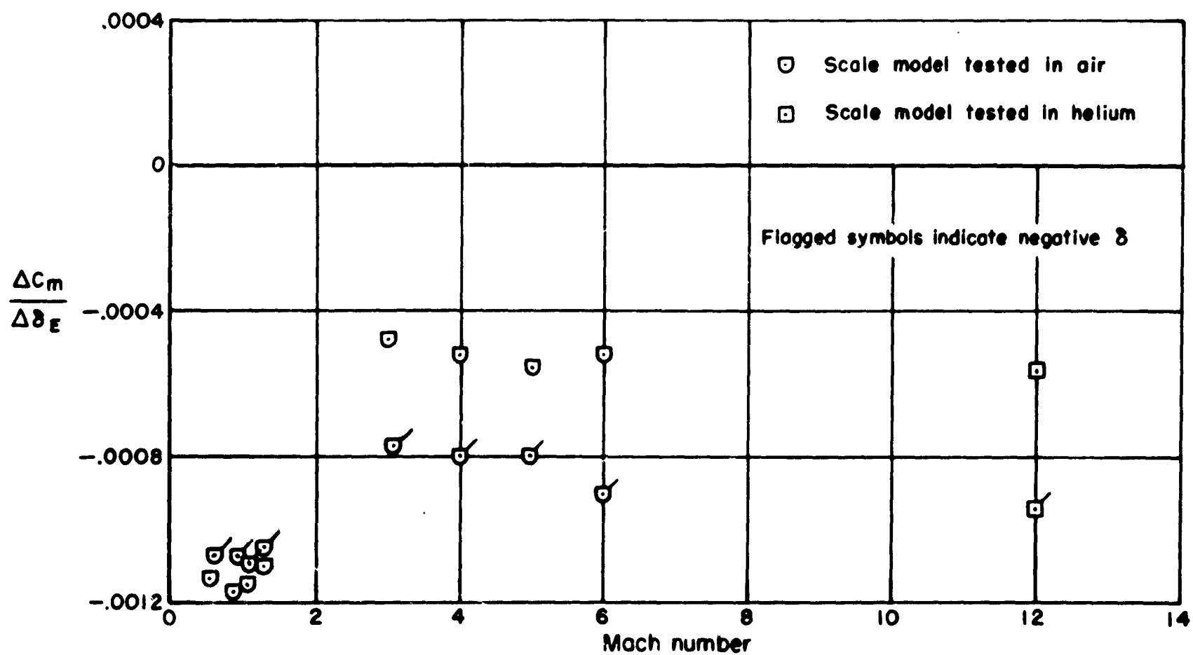
Figure 14.- Elevator effectiveness at \alpha = 5^\circ .
