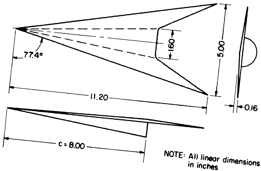
(a) Asymmetric model.
