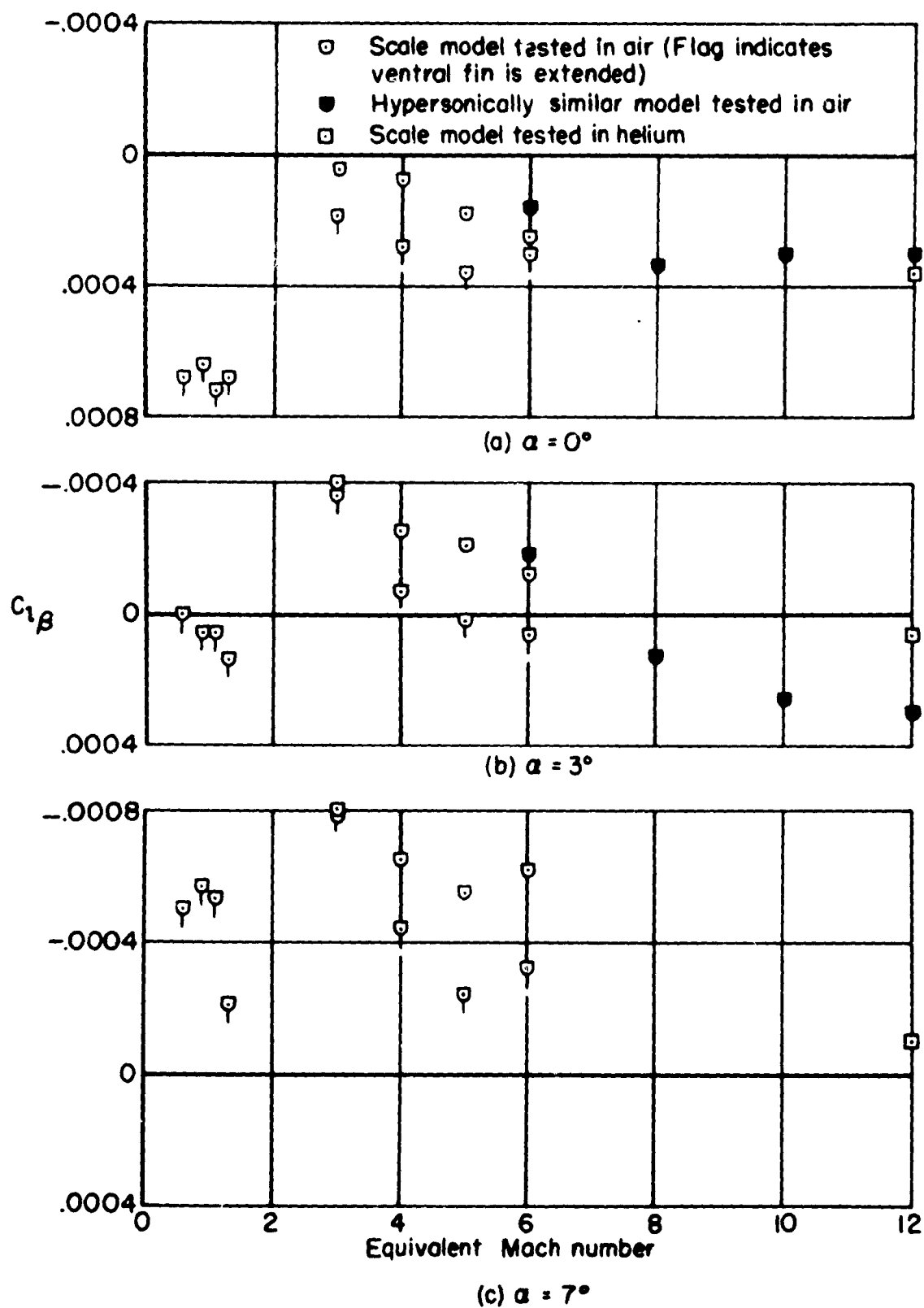
Figure 16.- Lateral-stability characteristics of glider.
