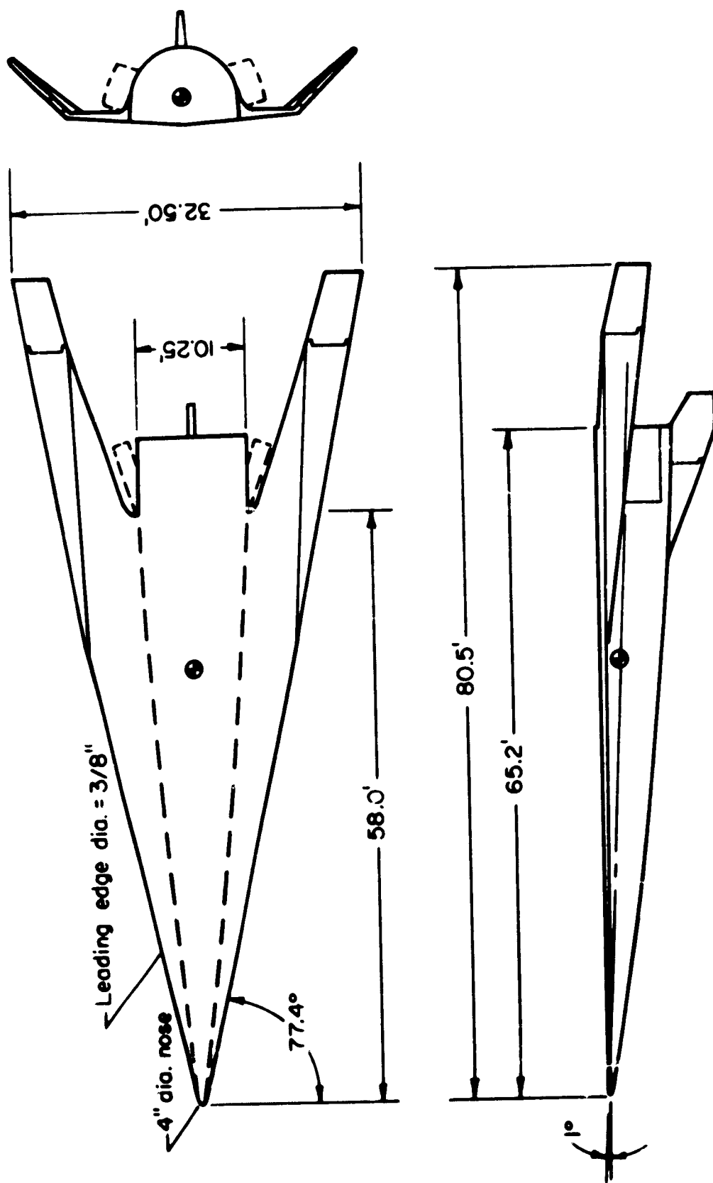
Figure 8.- Glider configuration.
