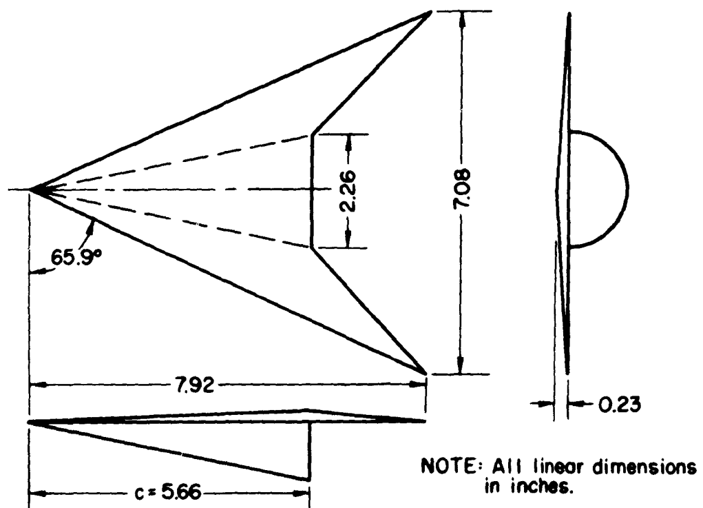
(a) Asymmetric model.
