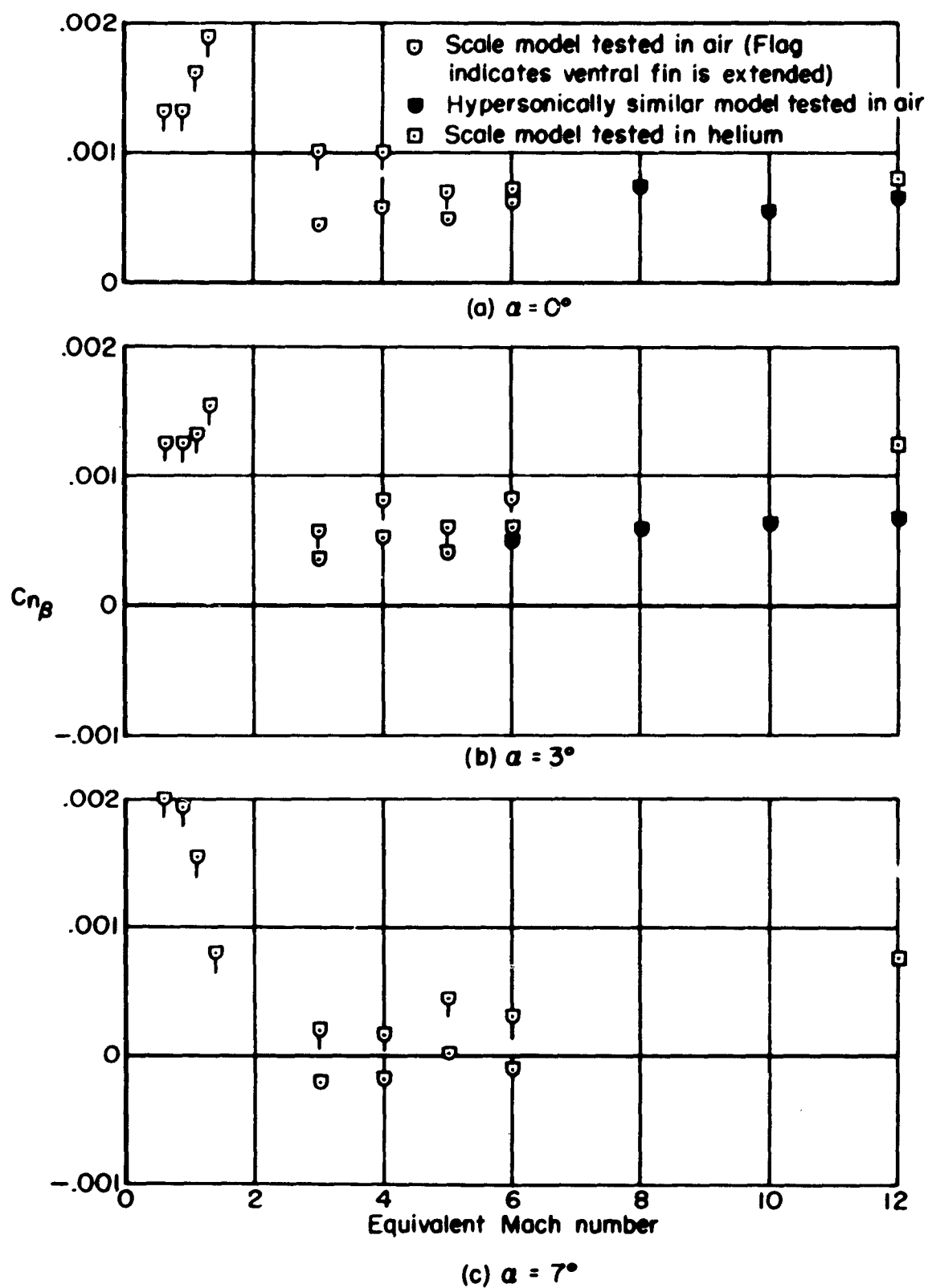
Figure 15.- Directional-stability characteristics of glider.
